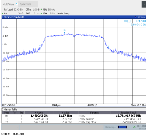
11g-Ant5-2452
