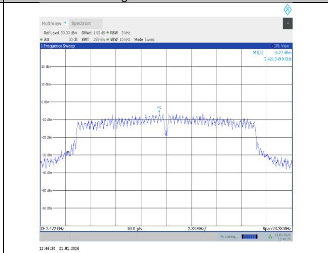
11g-Ant5-2422-PASS
