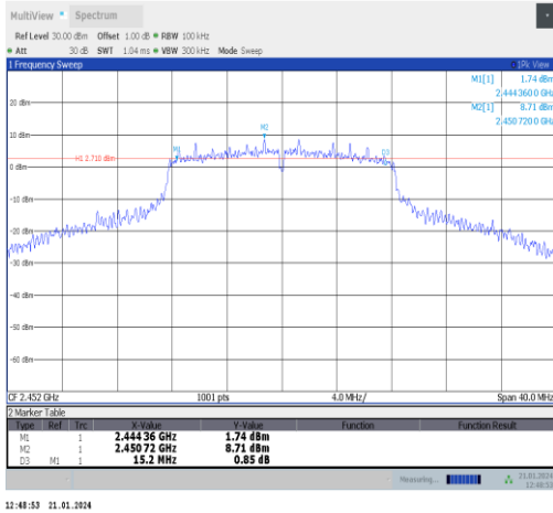
11g-Ant5-2452-PASS
