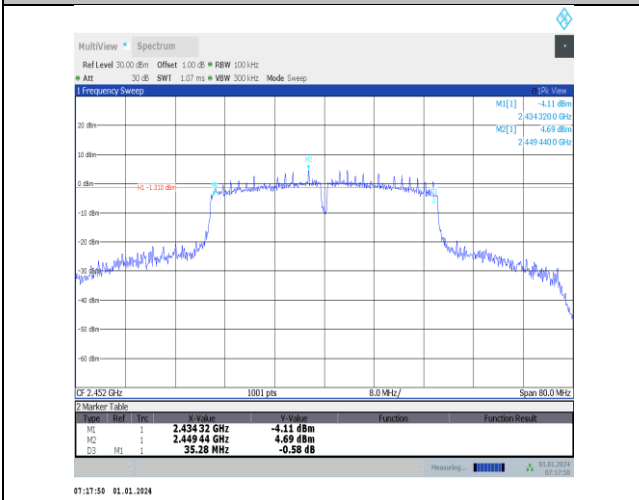
11n40SISO-Ant5-2452-PASS
