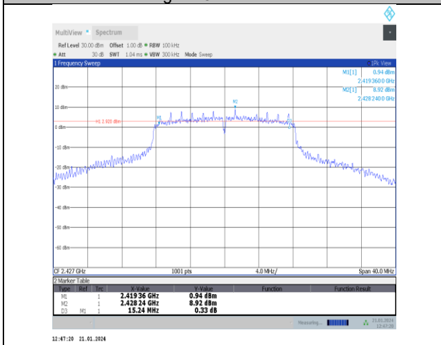
11g-Ant5-2427-PASS
