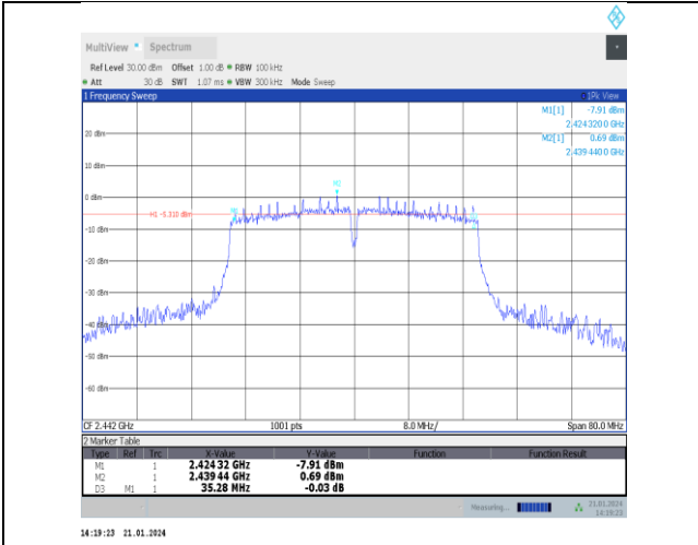
11n40SISO-Ant5-2442-PASS
