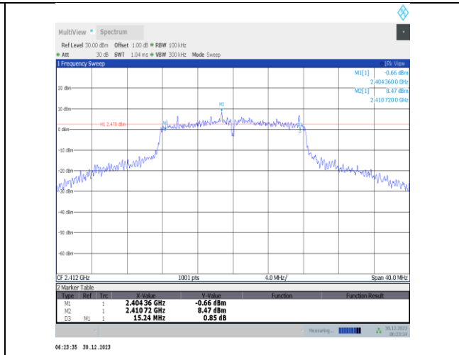
11g-Ant5-2412-PASS
