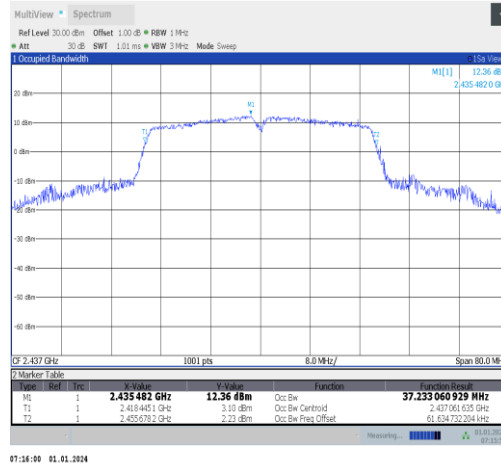
11n40SISO-Ant5-2437
