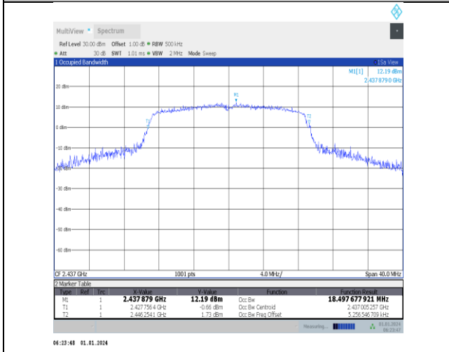
11n20SISO-Ant5-2437
