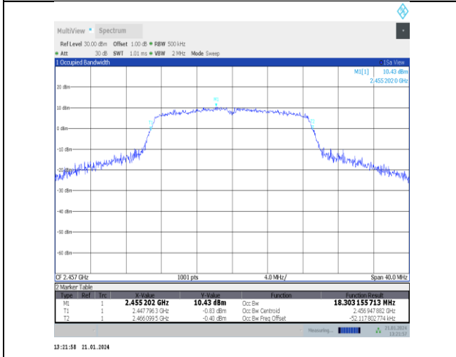
11n20SISO-Ant5-2457
