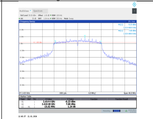
11g-Ant5-2422-PASS
