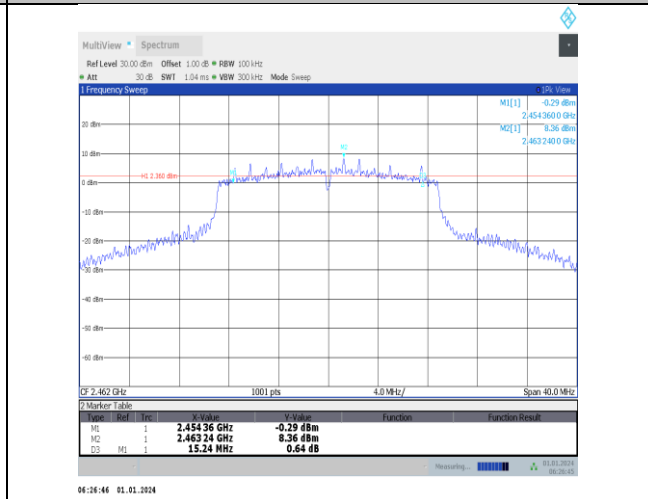
11n20SISO-Ant5-2462-PASS
