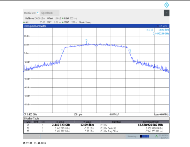
11n20SISO-Ant5-2452
