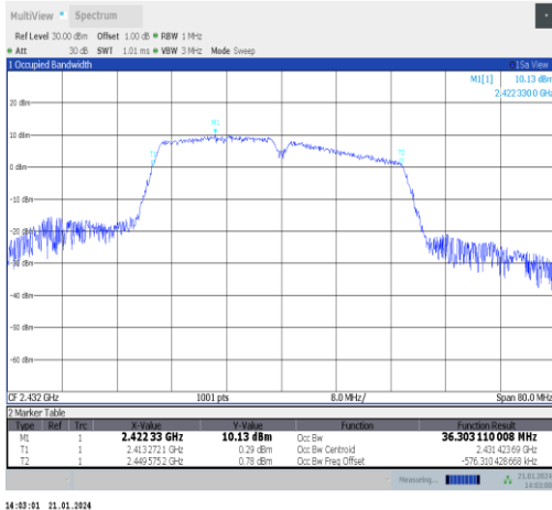
11n40SISO-Ant5-2432
