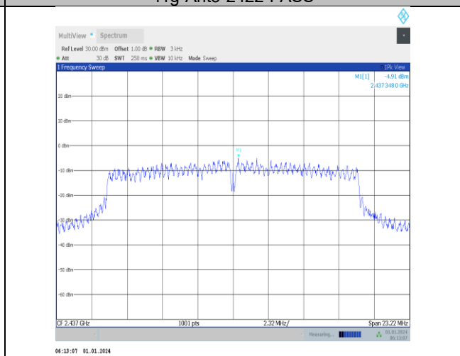
11g-Ant5-2437-PASS
