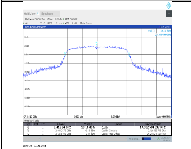
11g-Ant5-2417
