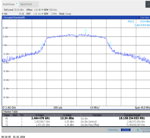
11g-Ant5-2462
