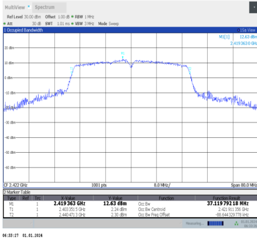
11n40SISO-Ant5-2422
