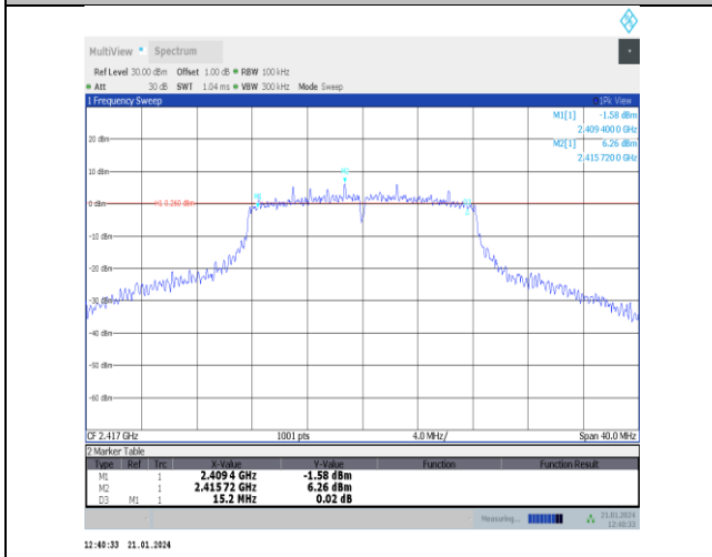
11g-Ant5-2417-PASS
