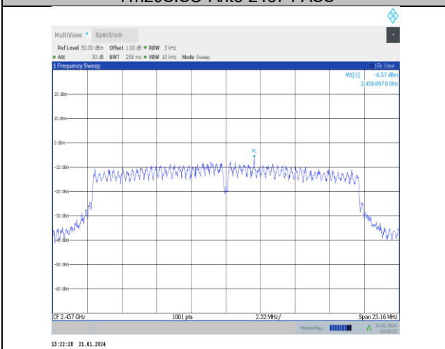
11n20SISO-Ant5-2457-PASS
