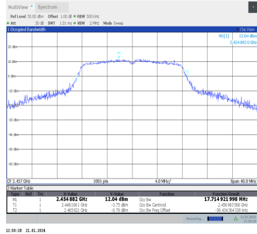
11g-Ant5-2457
