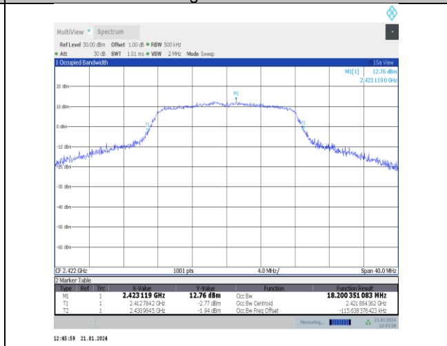
11g-Ant5-2422
