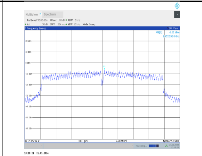
11n20SISO-Ant5-2452-PASS
