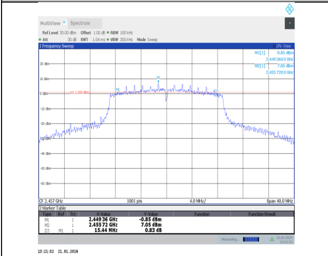
11n20SISO-Ant5-2457-PASS
