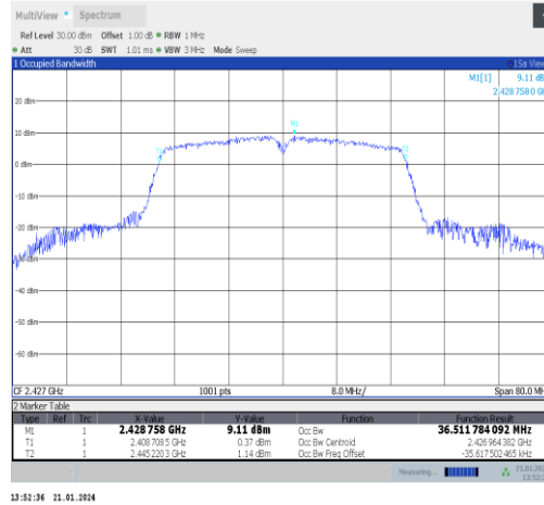
11n40SISO-Ant5-2427
