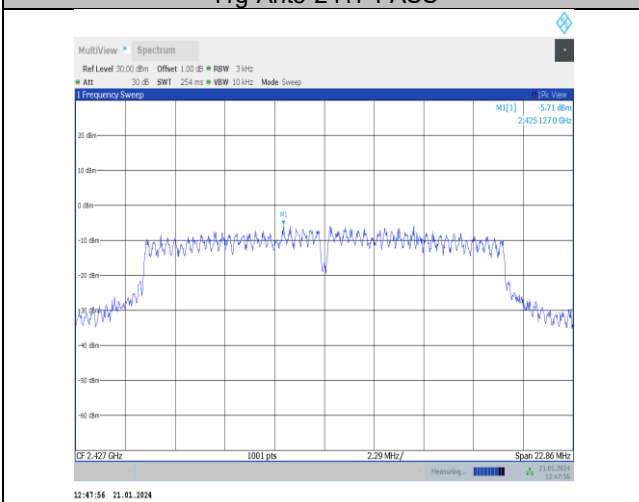
11g-Ant5-2427-PASS
