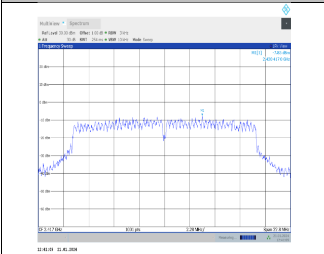
11g-Ant5-2417-PASS
