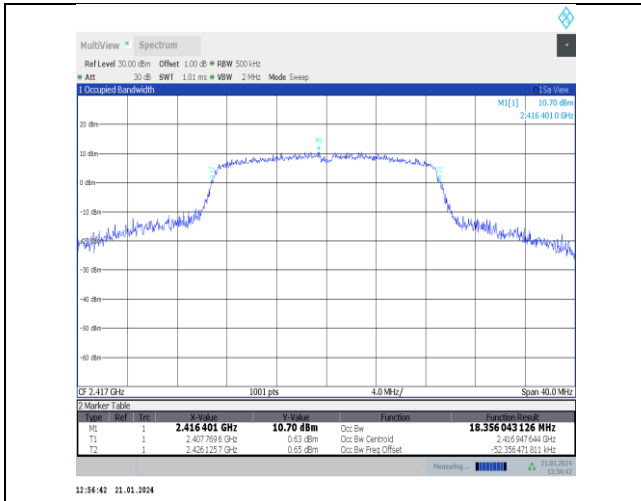
11n20SISO-Ant5-2417
