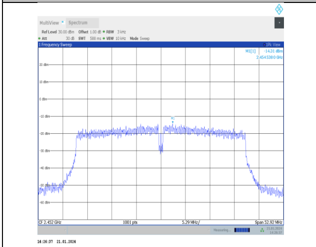
11n40SISO-Ant5-2452-PASS
