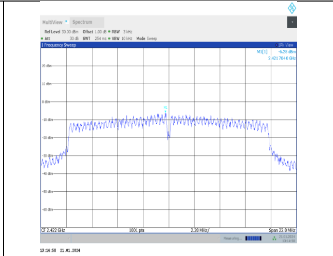
11n20SISO-Ant5-2422-PASS
