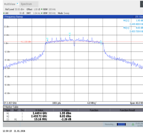
11g-Ant5-2457-PASS
