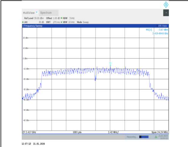
11n20SISO-Ant5-2417-PASS
