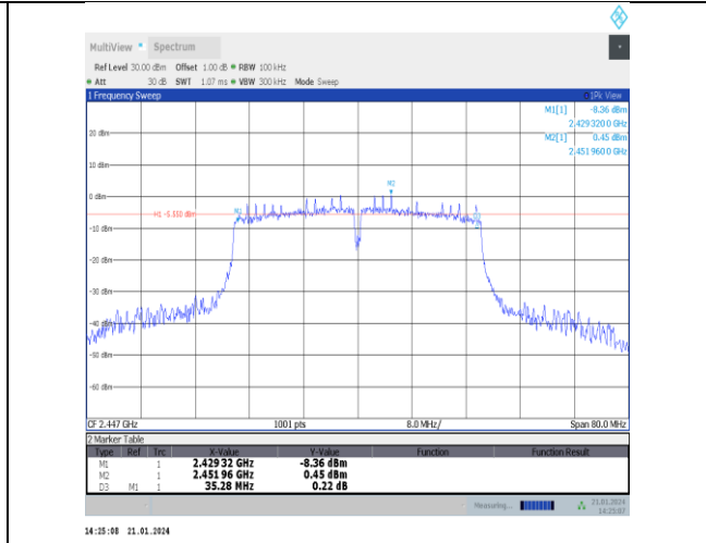
11n40SISO-Ant5-2447-PASS
