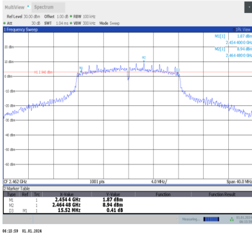
11g-Ant5-2462-PASS
