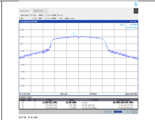
11n20SISO-Ant5-2422
