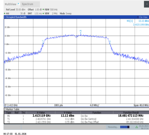
11n20SISO-Ant5-2412
