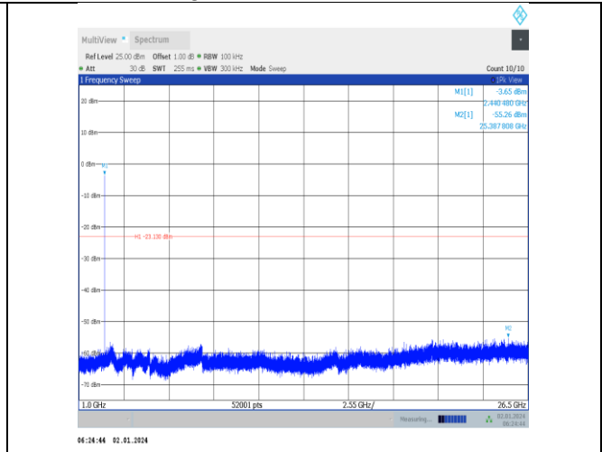
BLE_1M-Ant5-2440-1000~26500-PASS
