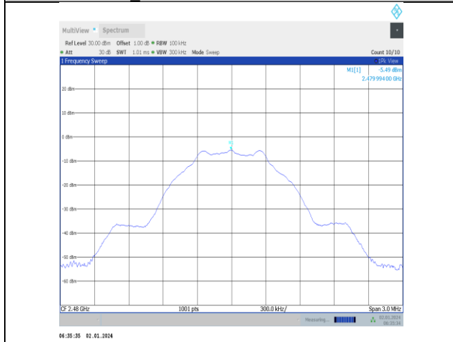
BLE_1M-Ant5-2480-0~Reference-PASS
