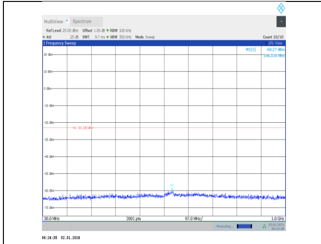
BLE_1M-Ant5-2440-30~1000-PASS
