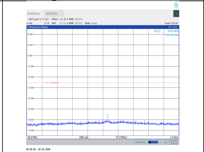
BLE_1M-Ant5-2480-30~1000-PASS
