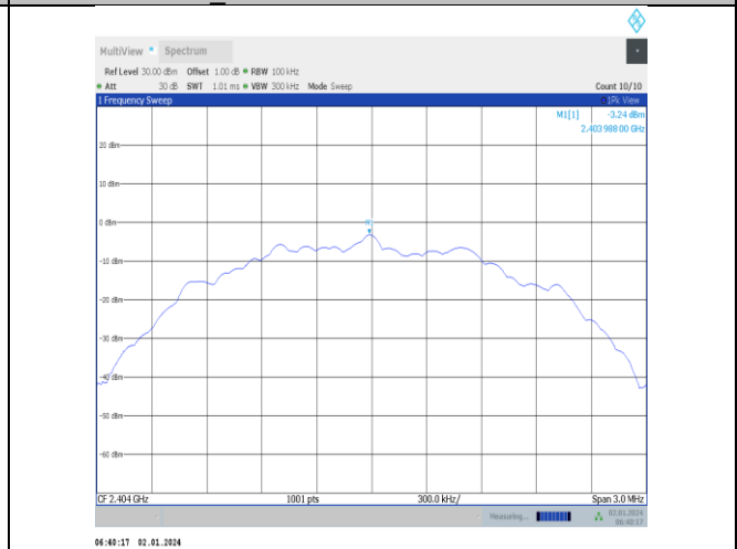
BLE_2M-Ant5-2404-0~Reference-PASS
