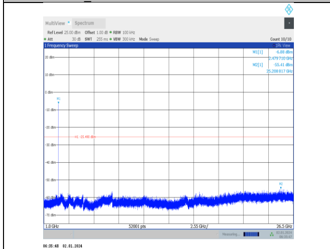
BLE_1M-Ant5-2480-1000~26500-PASS
