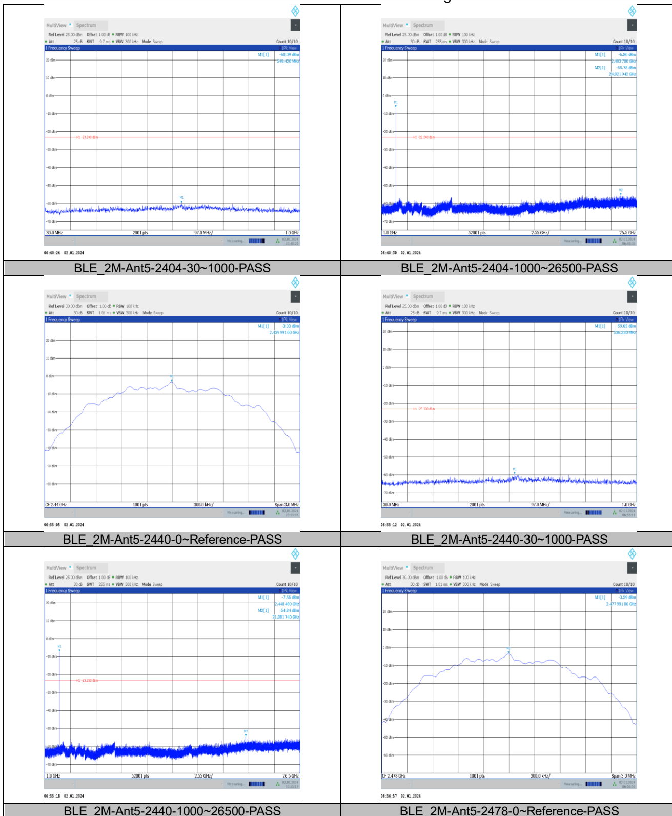
BLE_2M-Ant5-2440-1000~26500-PASS
