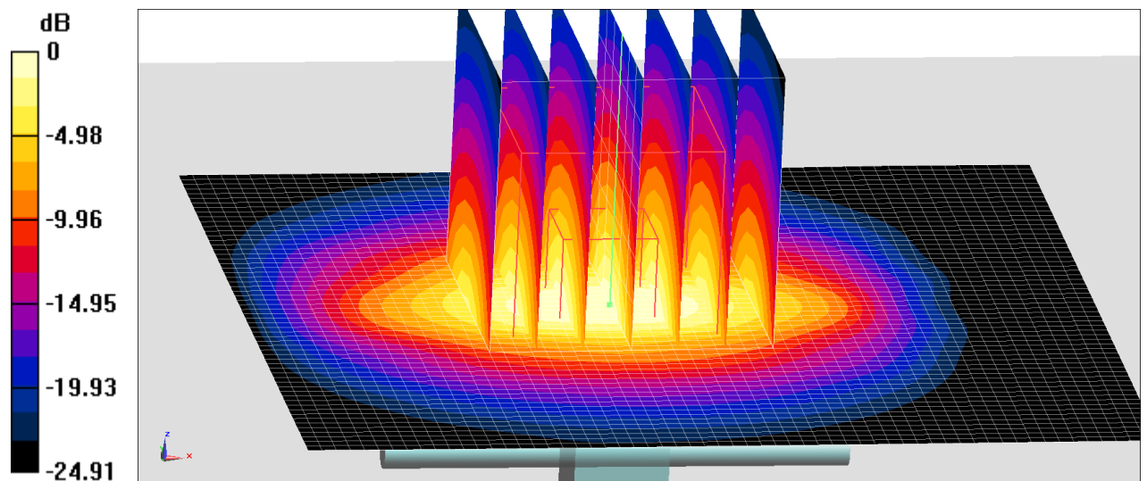
Fig.B.5 validation 2300MHz 250mW
