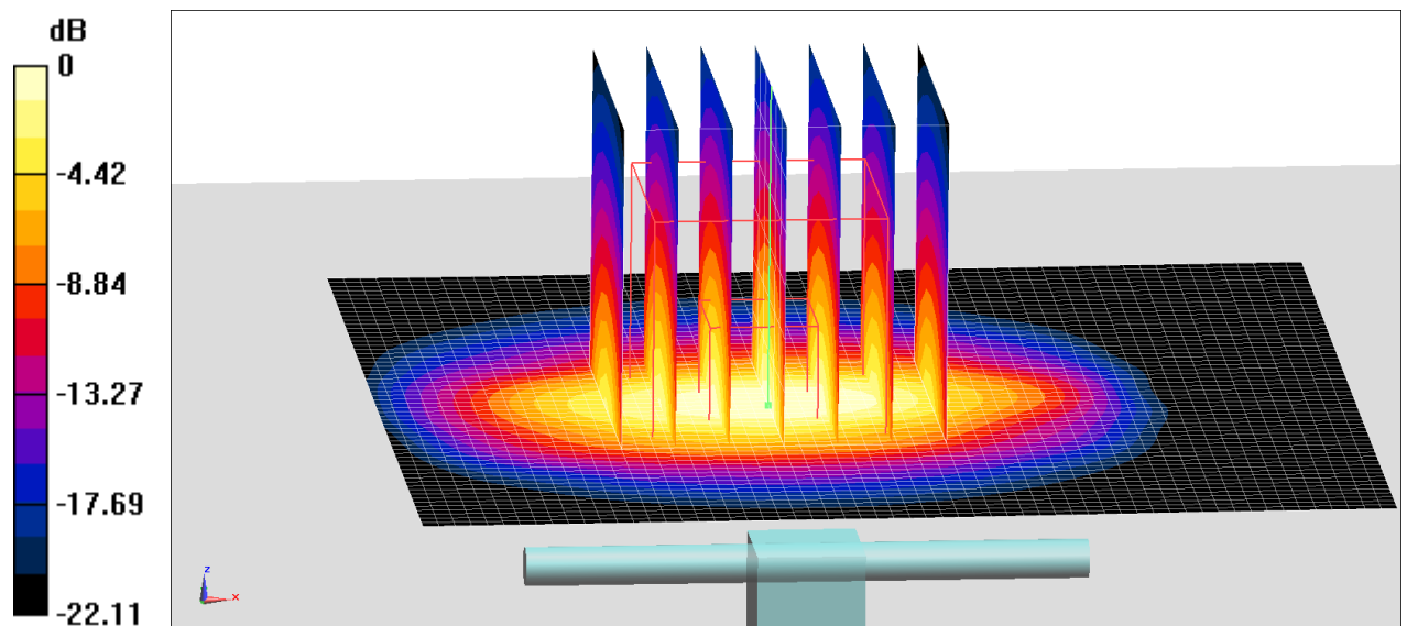
Fig.B.6 validation 2450MHz 250mW
