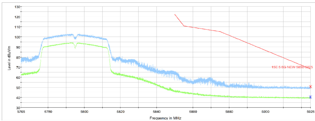
Fig. 6 Band Edges (802.11n-HT40 Ch159, 5795MHz)
