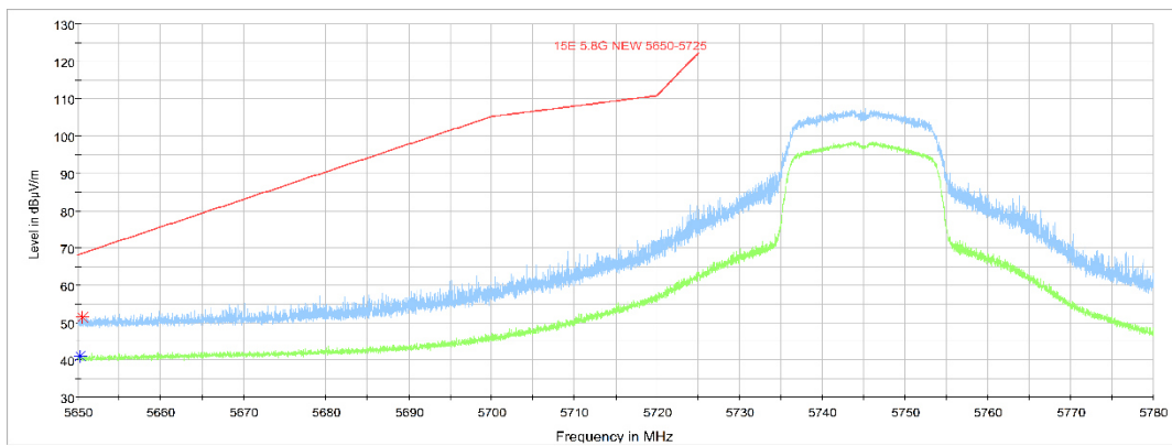
Fig. 3 Band Edges (802.11n-HT20 Ch149, 5745MHz)
