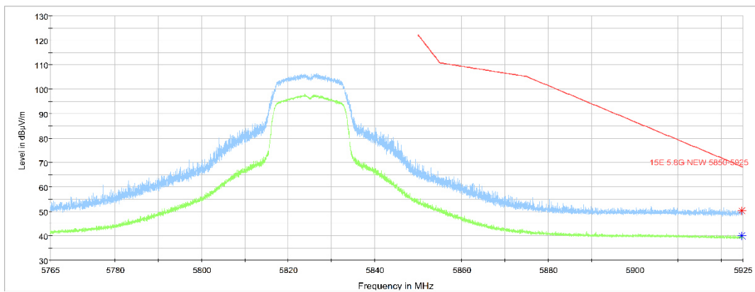
Fig. 2 Band Edges (802.11a Ch165, 5825MHz)
