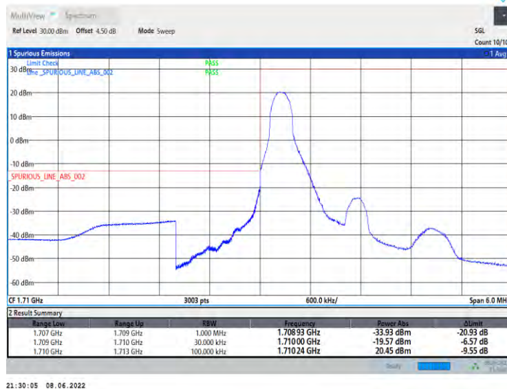
Band66-1.4MHz-QPSK-131979-6RB#0
