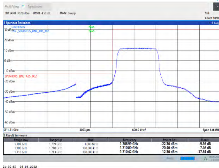
Band66-1.4MHz-QPSK-131979-6RB#0
