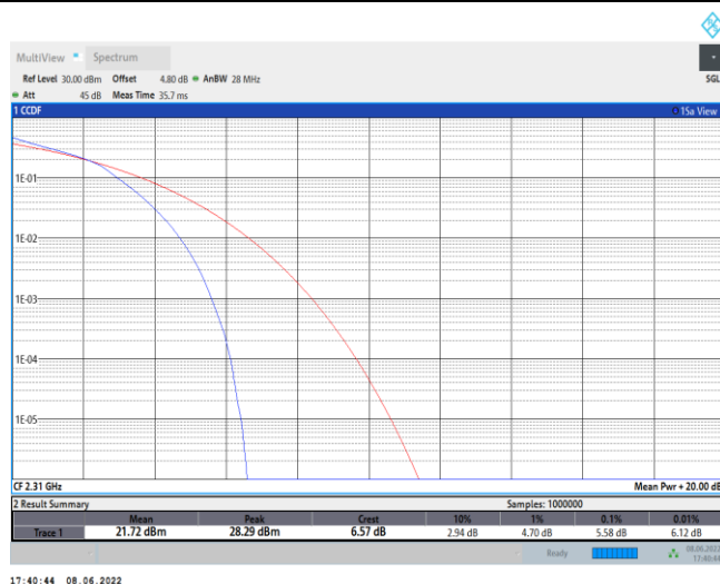
Band30-10MHz-16QAM-27710-50RB#0
