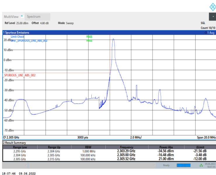
Band30-5MHz-QPSK-27685-25RB#0
