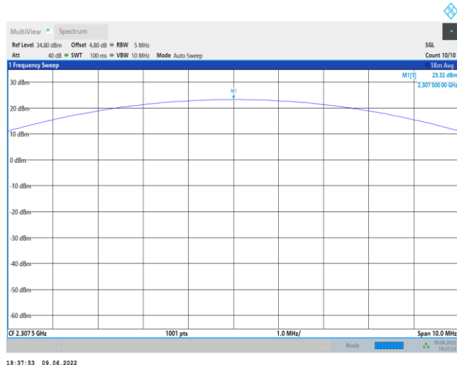
Band30-5MHz-QPSK-27685-1RB#12
