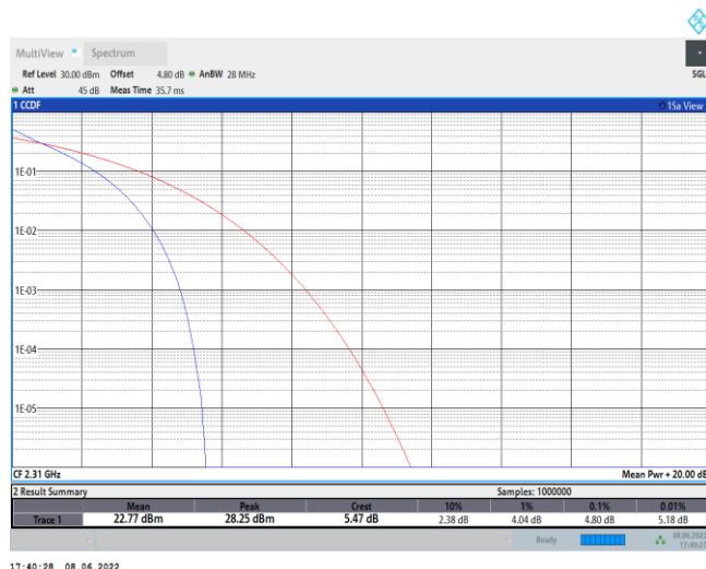
Band30-10MHz-16QAM-27710-50RB#0
