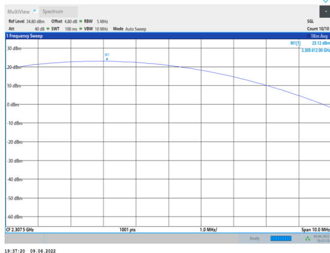
Band30-5MHz-QPSK-27685-1RB#12
