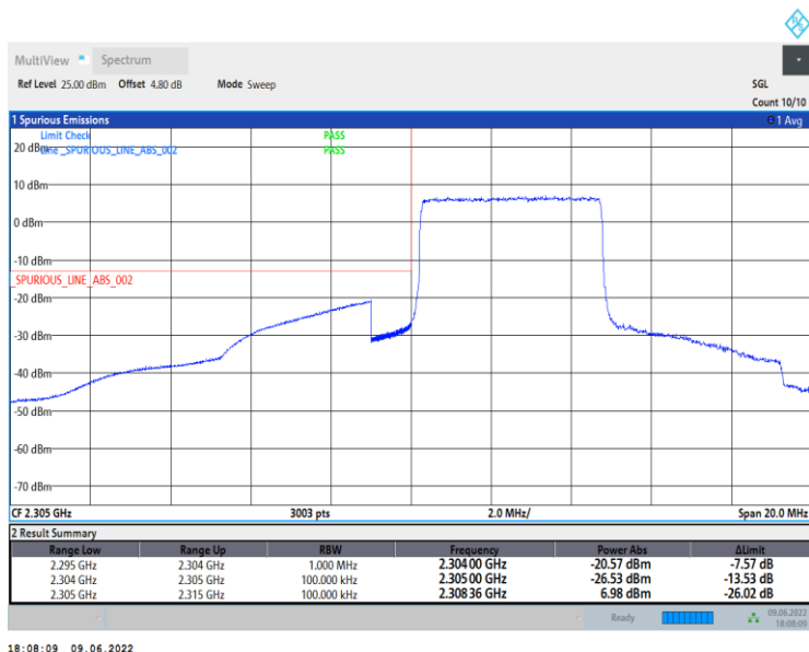
Band30-5MHz-QPSK-27685-25RB#0
