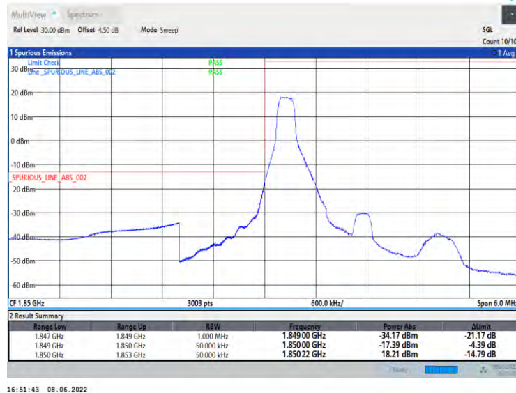
Band25-1.4MHz-QPSK-26047-6RB#0
