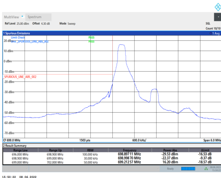
Band12-1.4MHz-QPSK-23017-6RB#0
