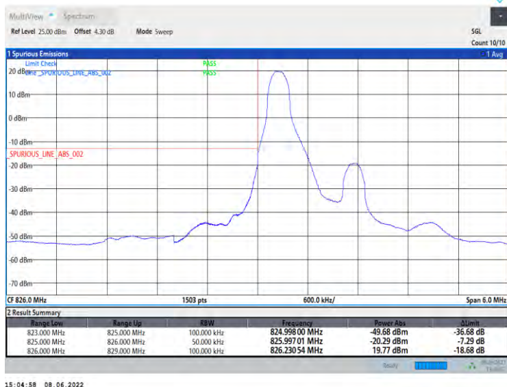
Band5-1.4MHz-QPSK-20427-6RB#0
