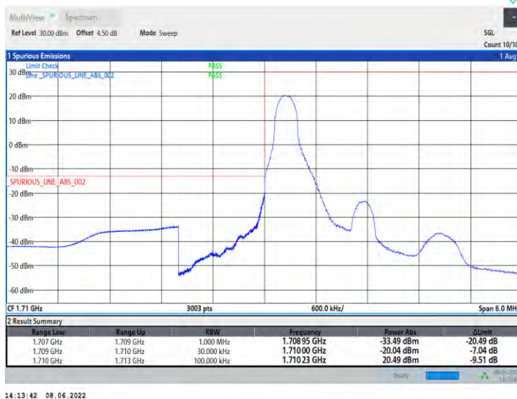
Band4-1.4MHz-QPSK-19957-6RB#0
