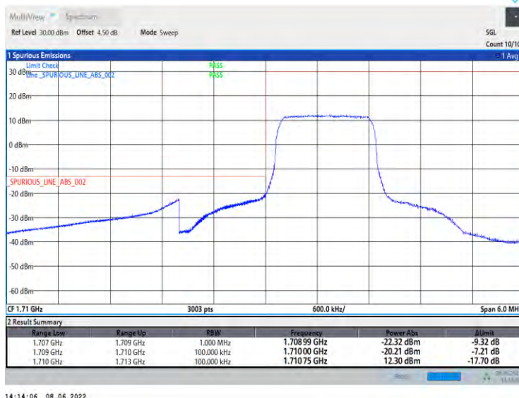
Band4-1.4MHz-QPSK-19957-6RB#0
