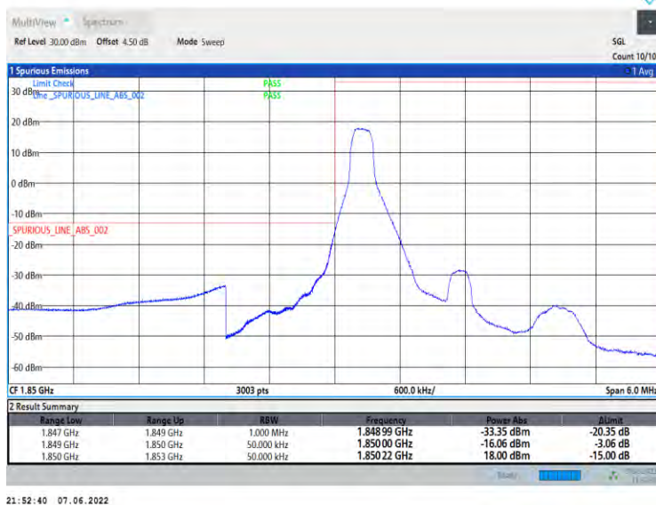
Band2-1.4MHz-QPSK-18607-6RB#0
