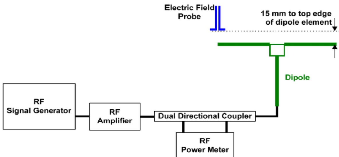
Fig.4 System verification
