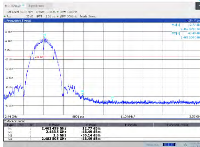
11B_Ant3_High_2462
