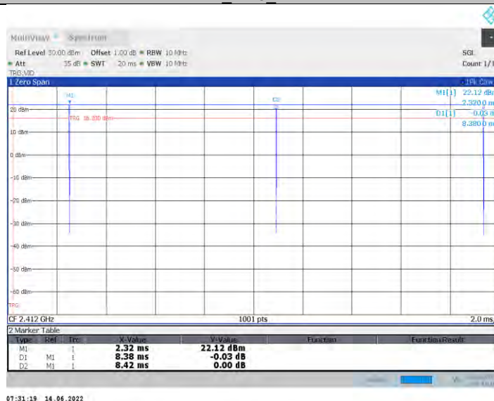
11G_Ant3_2412
