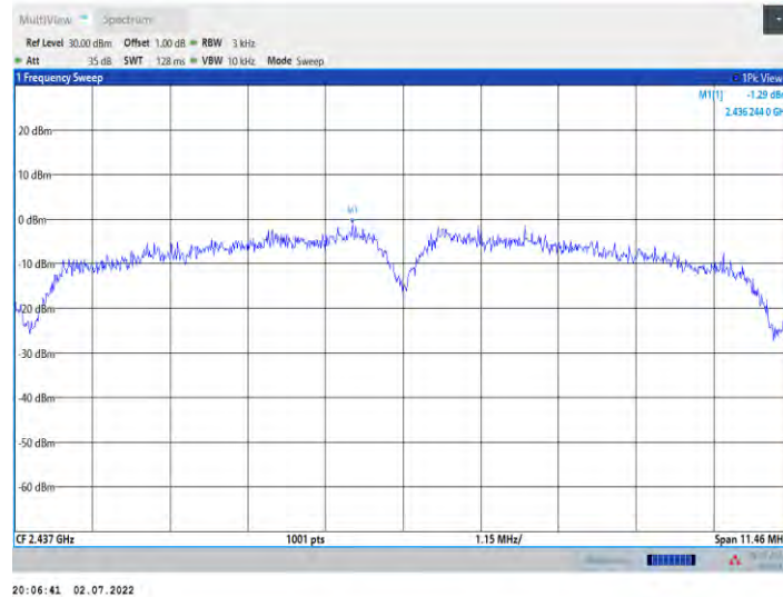
11B_Ant3_2437
