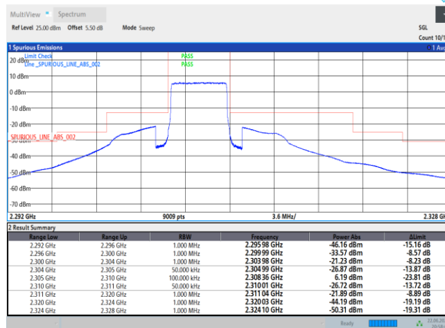
Band30-5MHz-QPSK-27685-25RB#0
