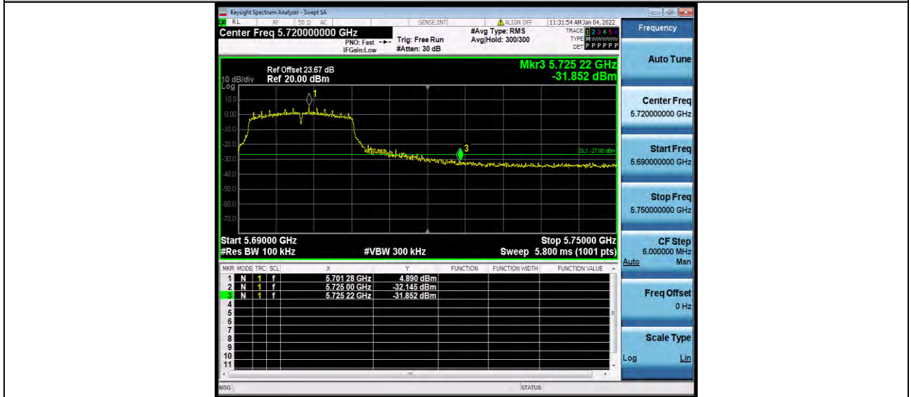
11A_Ant1_High_5700
