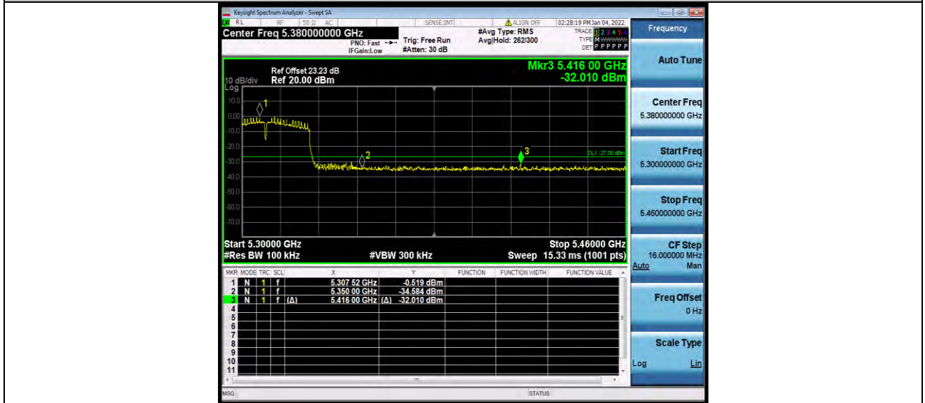
11N40SISO_Ant1_High_5310
