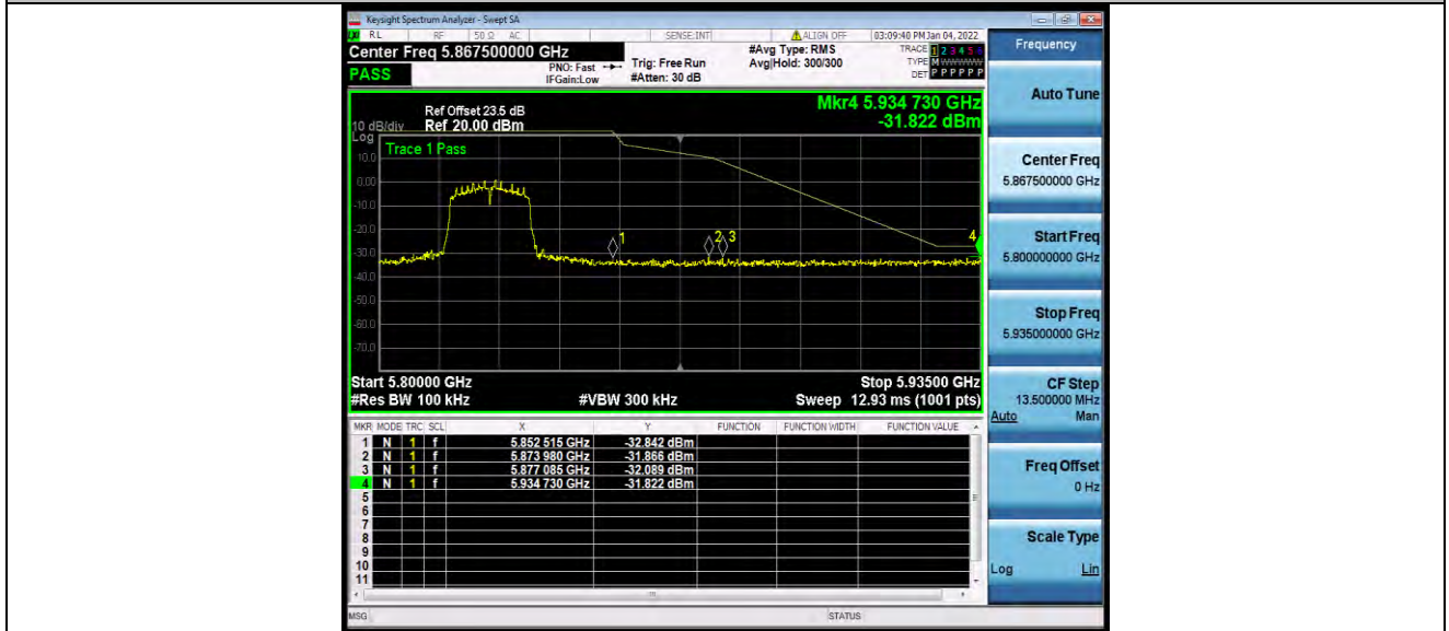
11AC20SISO_Ant1_High_5825
