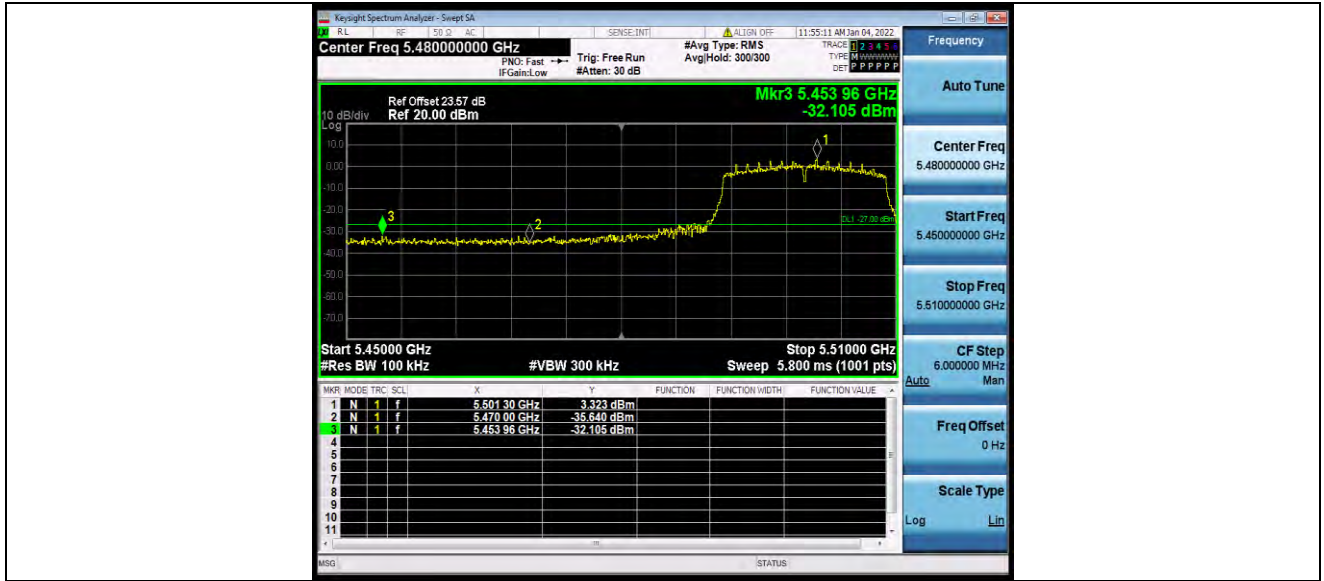
11N20SISO_Ant1_Low_5500
