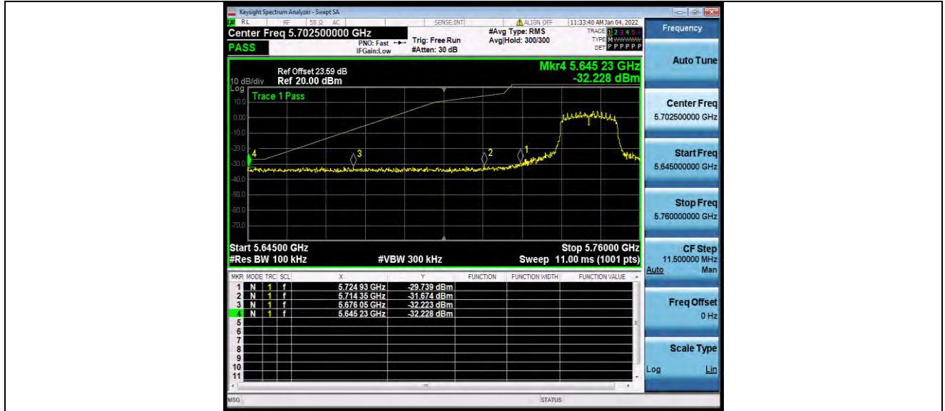
11A_Ant1_Low_5745
