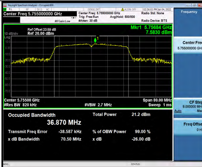
11N40SISO_Ant1_5755
