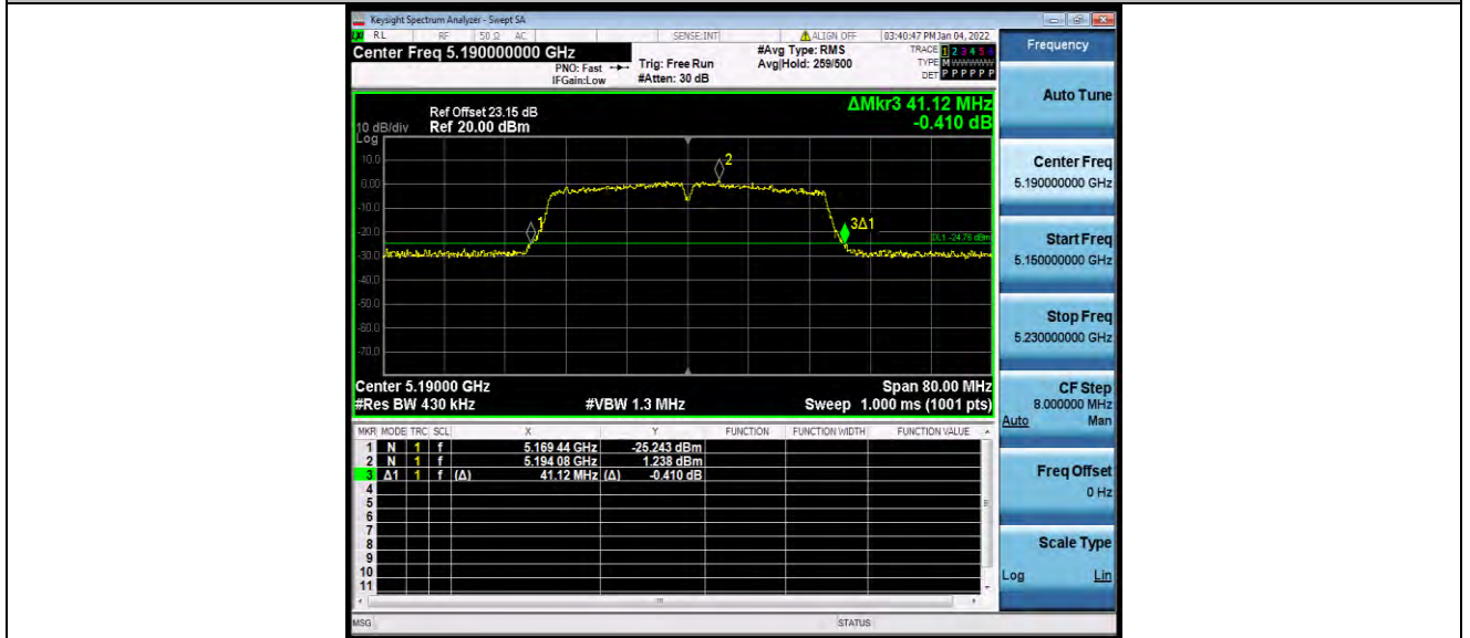
11AC40SISO_Ant1_5190
