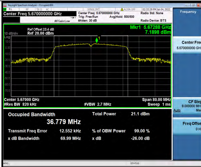
11N40SISO_Ant1_5670
