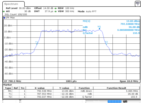
Lowest Channel / 5MHz / 16QAM
