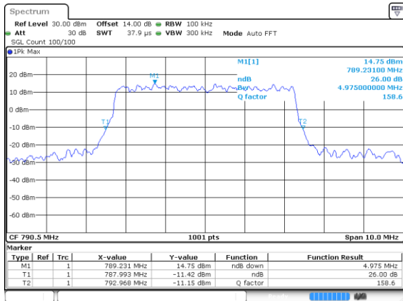
Lowest Channel / 5MHz / QPSK
