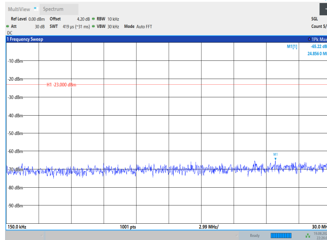
Band26-15MHz-QPSK-26865-1RB#0-Range2:0.15~30MHz
