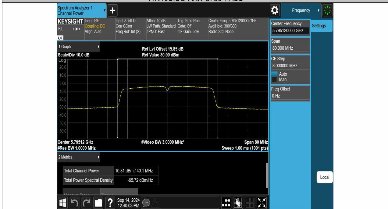
11N40SISO-Ant1-5795-PASS
