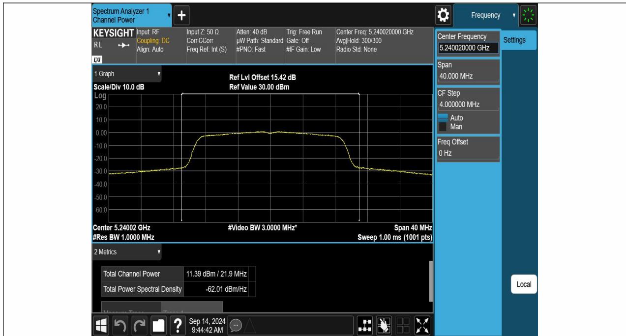
11N20SISO-Ant1-5240-PASS
