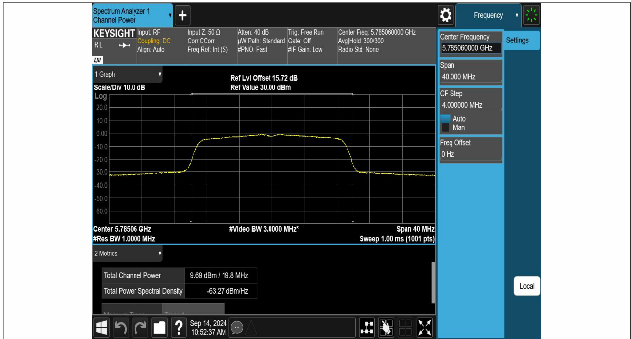
11N20SISO-Ant1-5785-PASS
