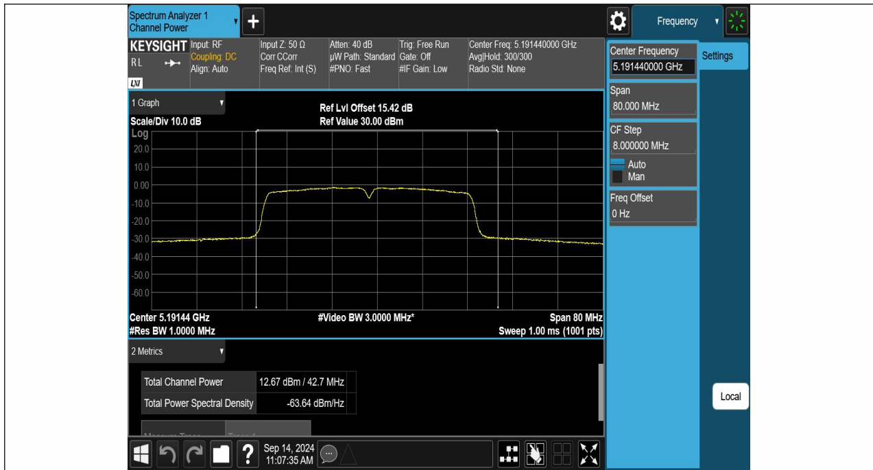
11N40SISO-Ant1-5190-PASS
