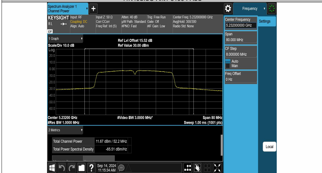
11N40SISO-Ant1-5230-PASS
