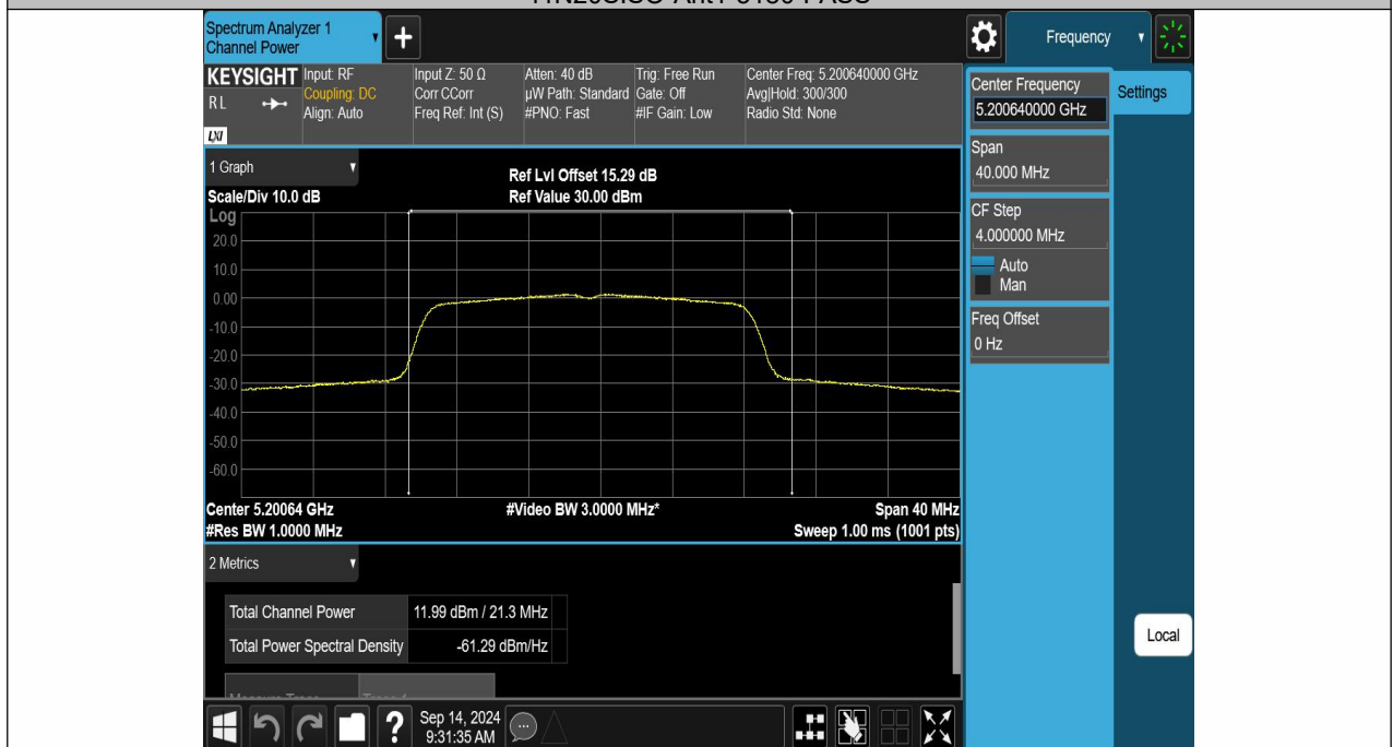
11N20SISO-Ant1-5200-PASS
