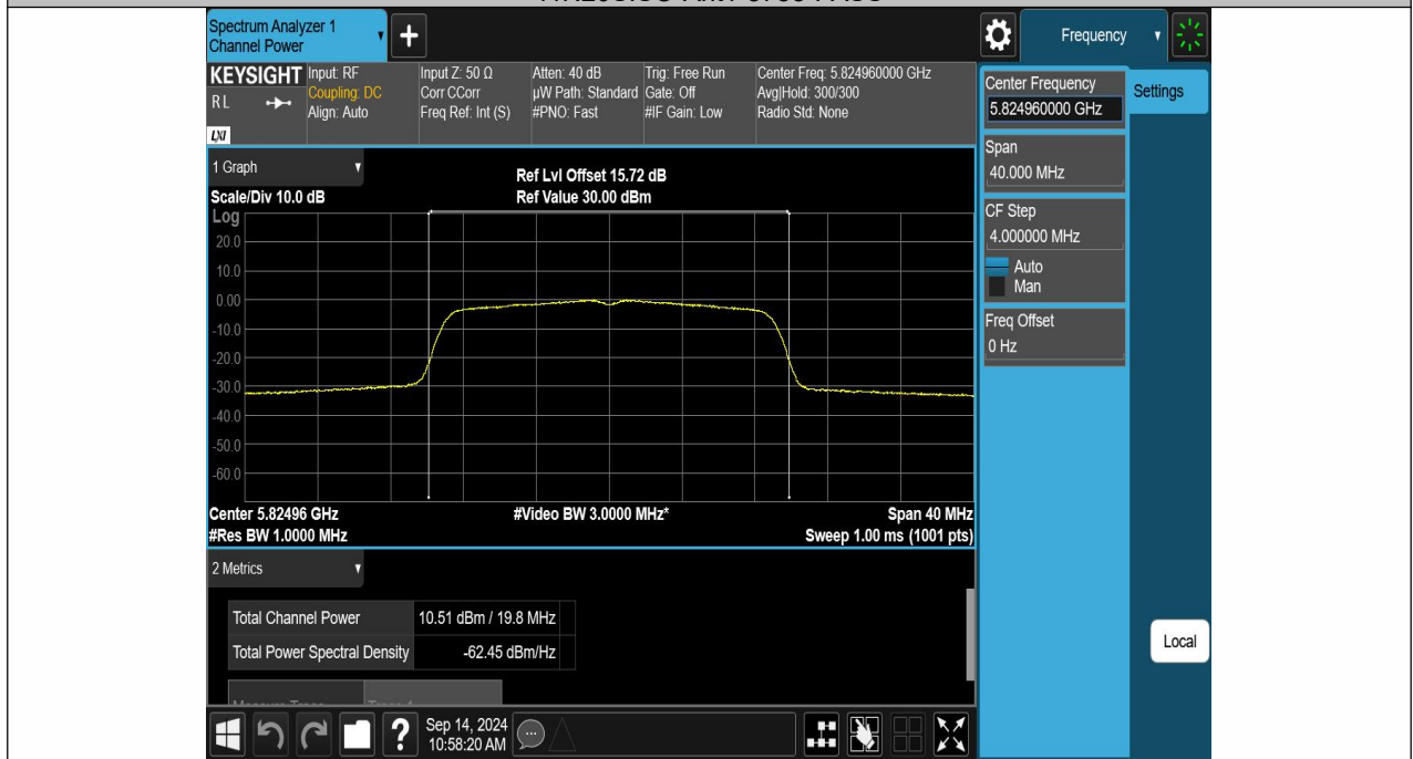
11N20SISO-Ant1-5825-PASS
