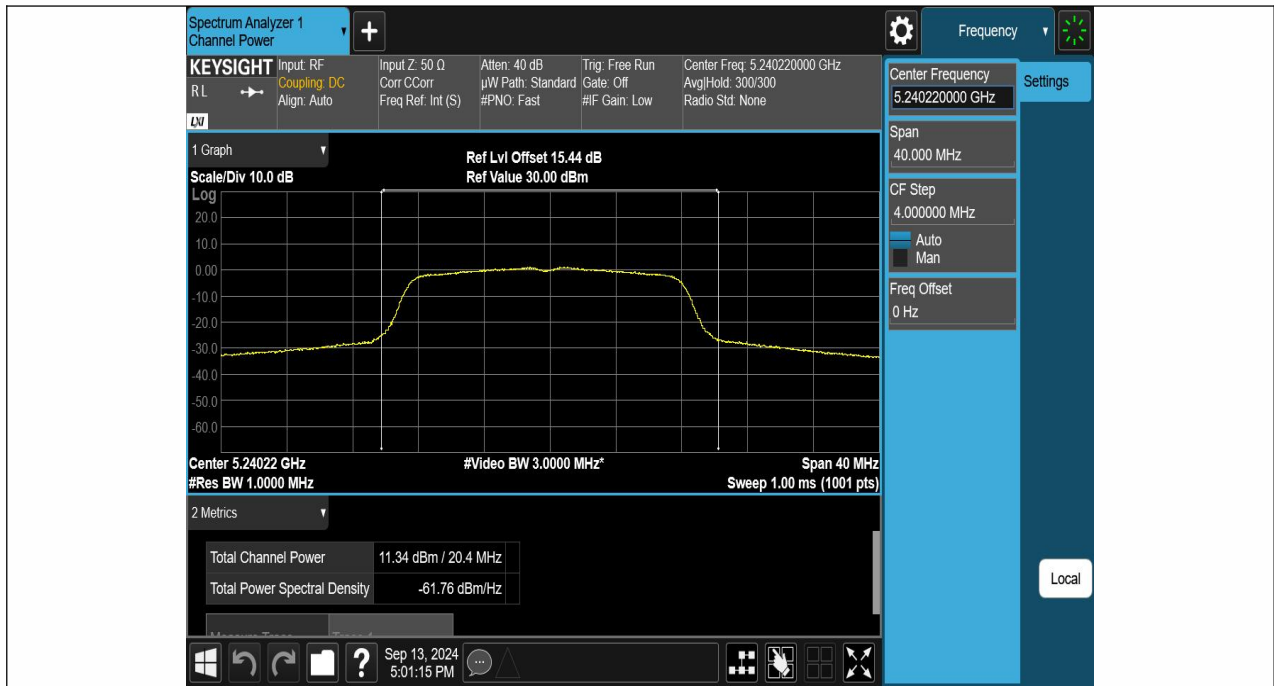
11A-Ant1-5240-PASS
