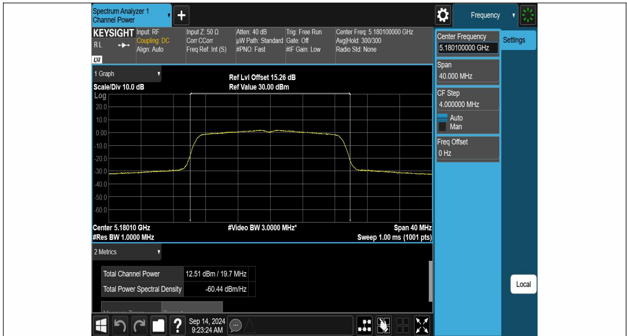
11N20SISO-Ant1-5180-PASS
