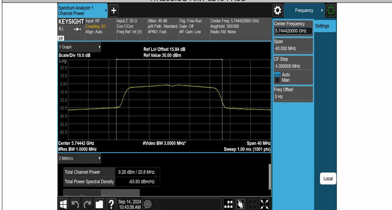
11N20SISO-Ant1-5745-PASS
