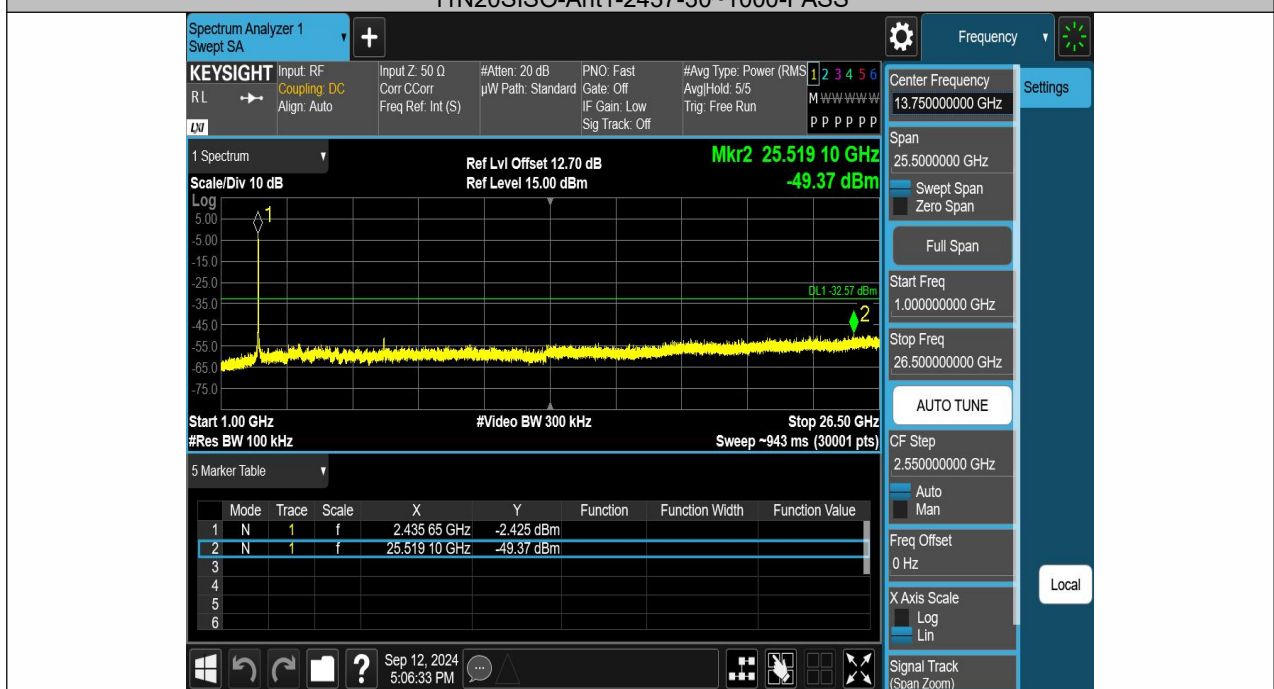
11N20SISO-Ant1-2437-1000~26500-PASS
