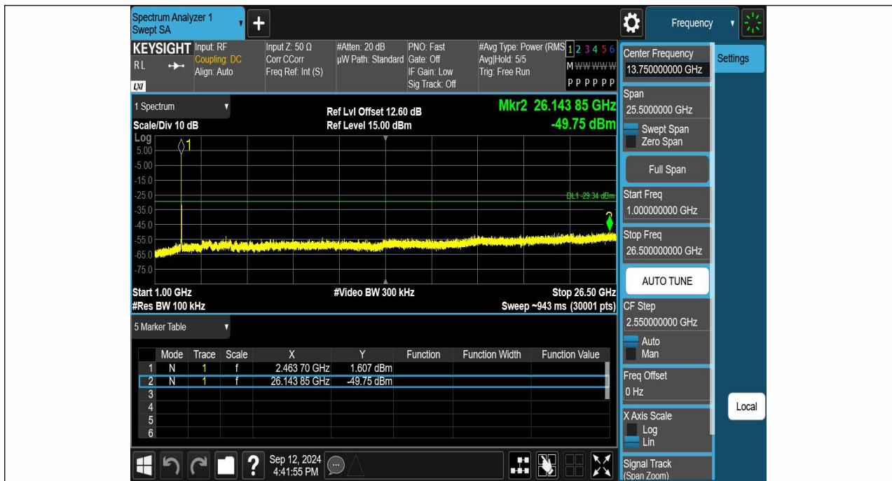
11B-Ant1-2462-1000~26500-PASS
