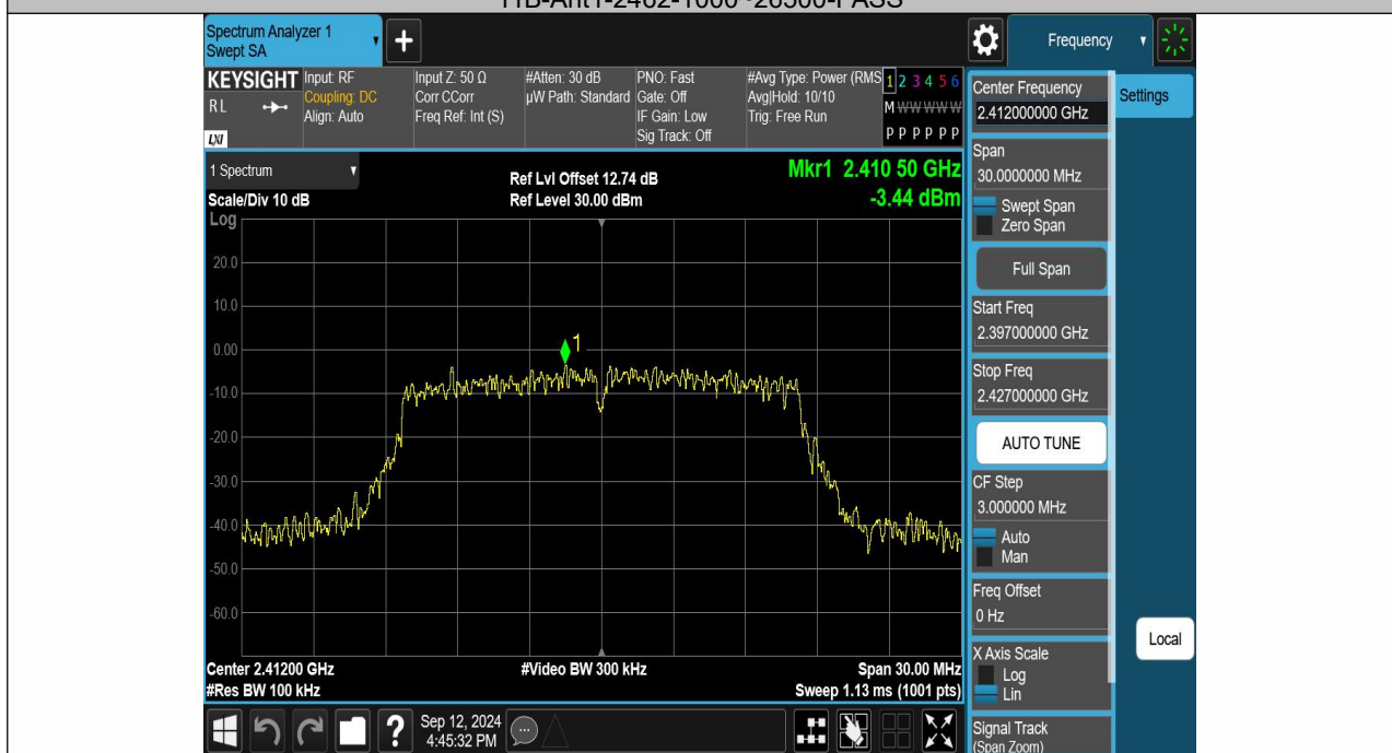
11G-Ant1-2412-0~Reference-PASS
