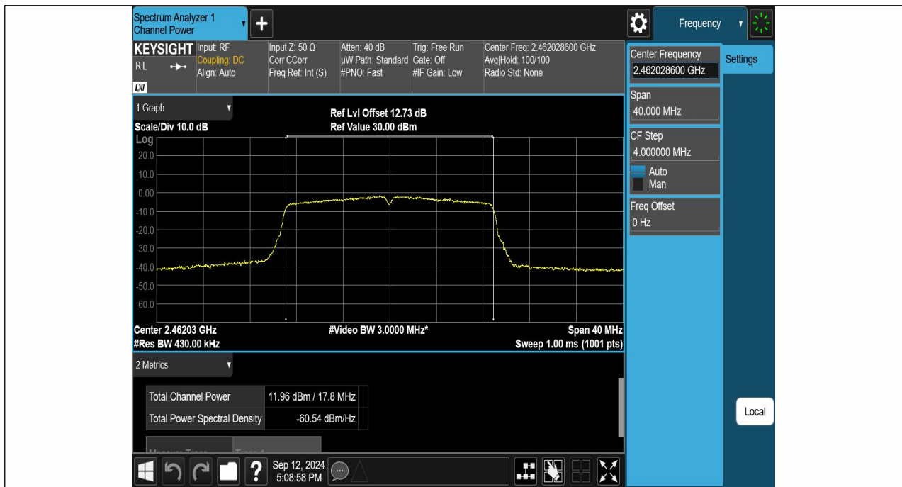
11N20SISO-Ant1-2462-PASS
