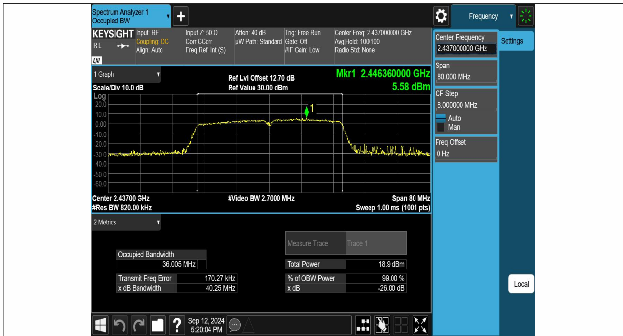
11N40SISO-Ant1-2437
