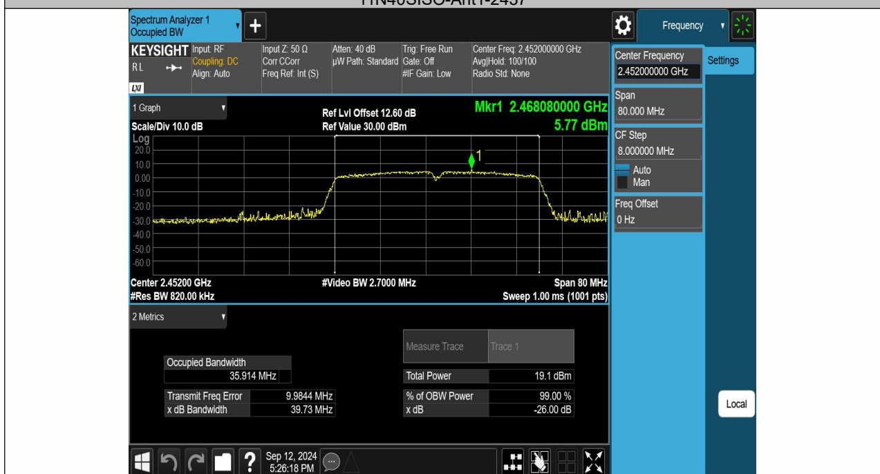
11N40SISO-Ant1-2452
