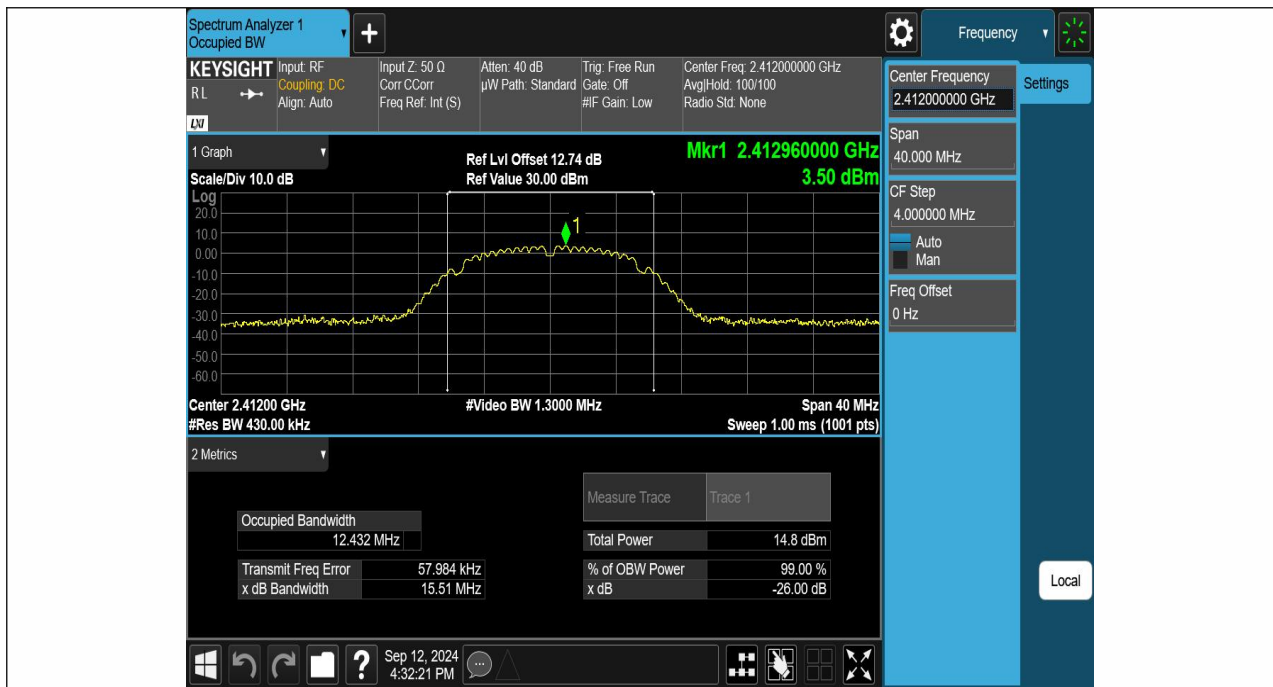
11B-Ant1-2412
