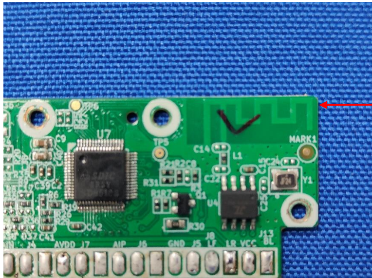
Bluetooth Antenna
