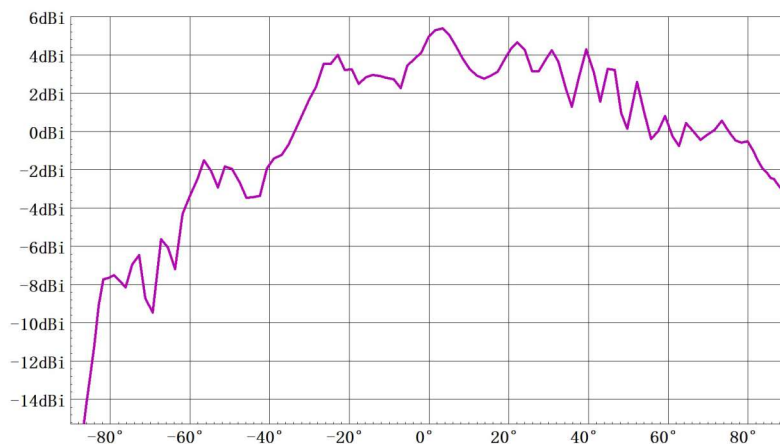
俯仰面方向图 (TX1) Freq:59.0GHz
