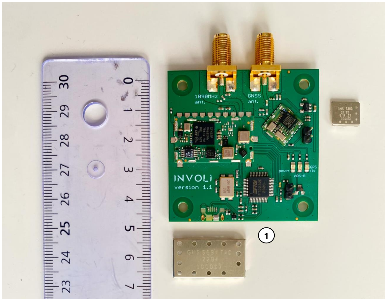
Figure 4: 1090 GNS 5894T receiver
