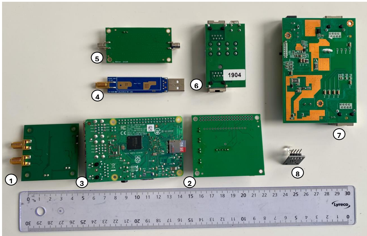
Figure 3: PCB bottom view
