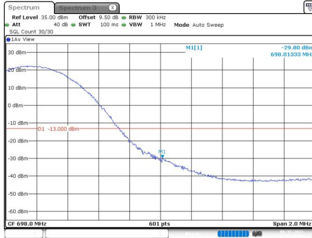
Band71-15MHz-16QAM-133397-1RB#74
