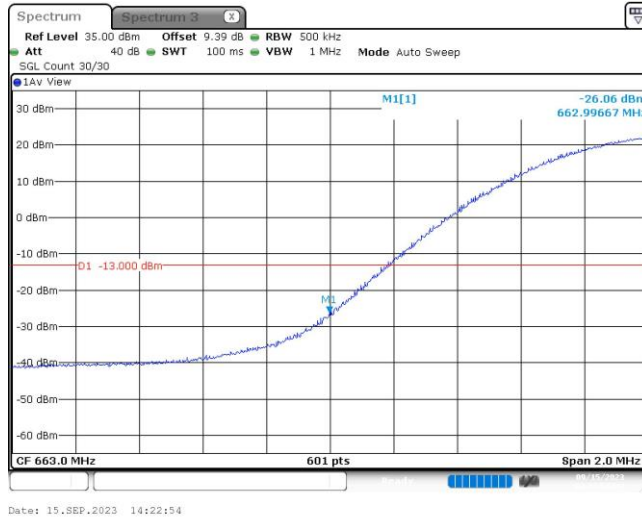
Band71-20MHz-16QAM-133222-1RB#99
