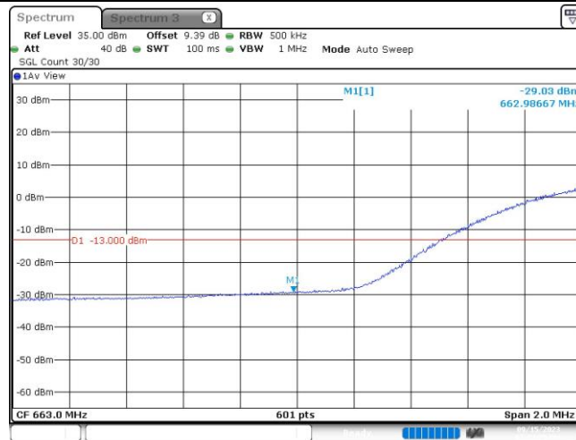
Band71-20MHz-QPSK-133222-100RB#0
