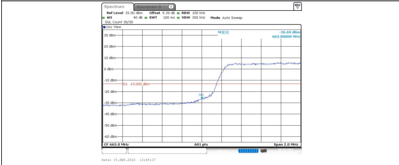
Band71-5MHz-16QAM-133447-1RB#0
