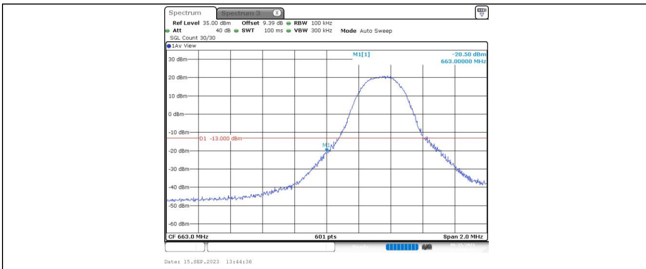
Band71-5MHz-16QAM-133147-1RB#24
