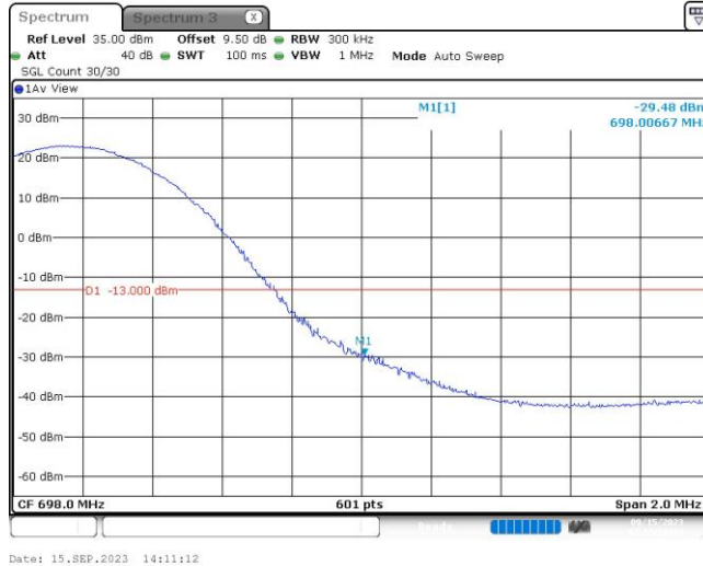
Band71-15MHz-QPSK-133397-75RB#0
