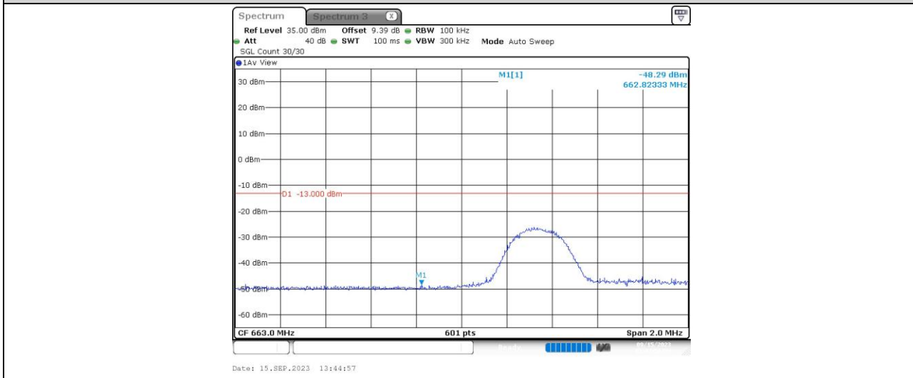
Band71-5MHz-16QAM-133147-25RB#0
