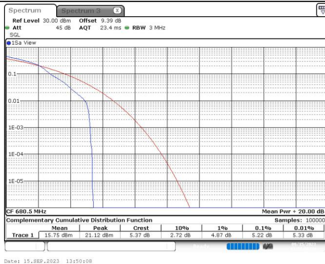
Band71-5MHz-16QAM-133297-25RB#0
