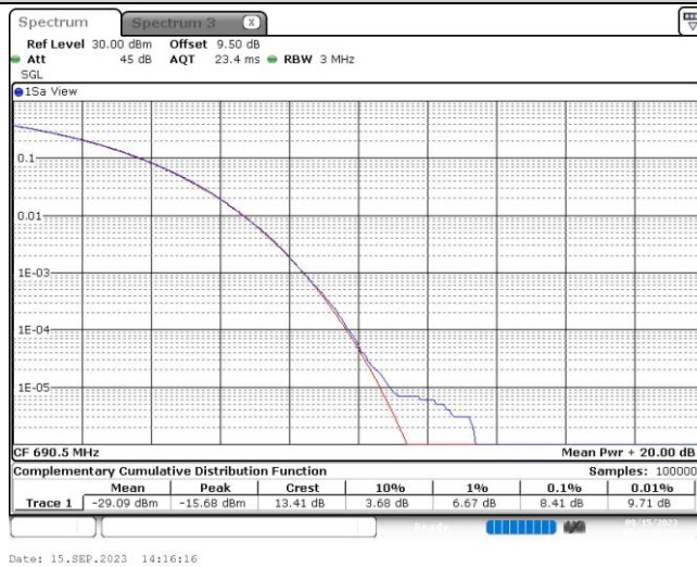
Band71-15MHz-16QAM-133397-75RB#0
