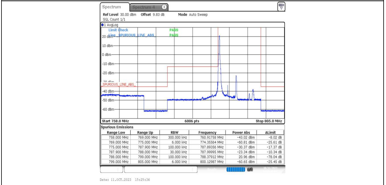
Band14_5MHz_16QAM_23305_1RB#0
