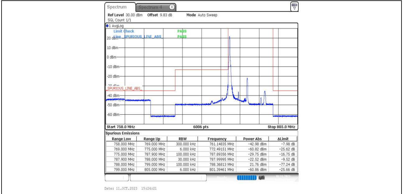
Band14_5MHz_QPSK_23305_1RB#0
