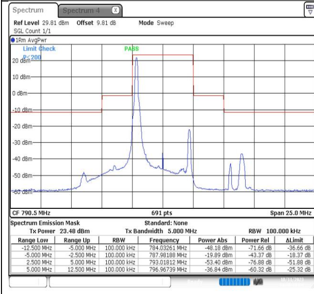
NTNV-Band14-5MHz-QPSK-23305-1RB#0--12.50--5.00-PASS
