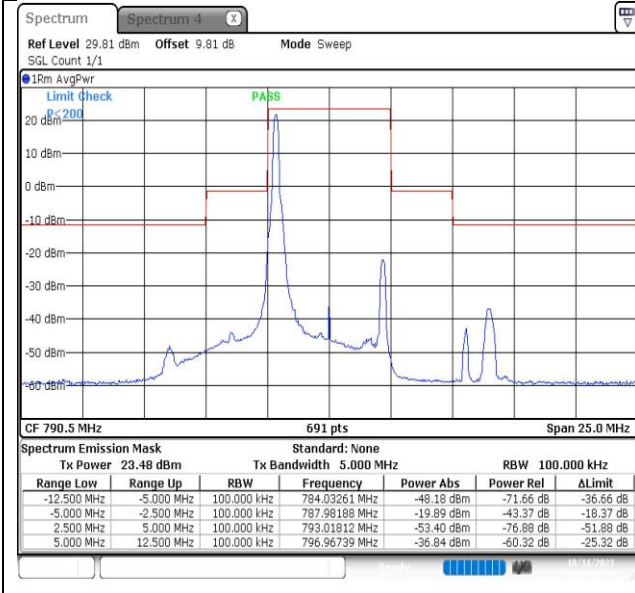
NTNV-Band14-5MHz-QPSK-23305-1RB#0--12.50--5.00-PASS
