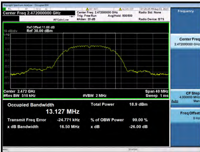
802.11b CHANNEL 13
