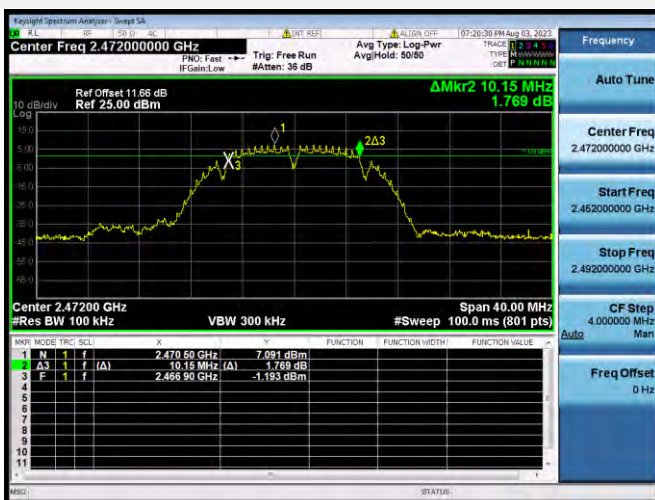
802.11b CHANNEL 13
