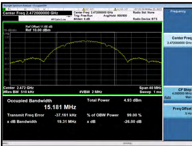
802.11b CHANNEL 13
