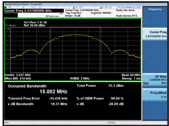
802.11b CHANNEL 6
