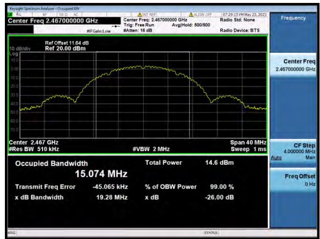
802.11b CHANNEL 12
