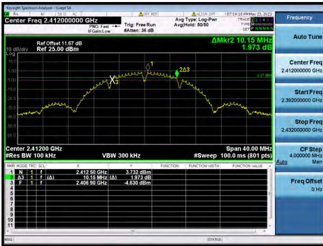
802.11b CHANNEL 1
