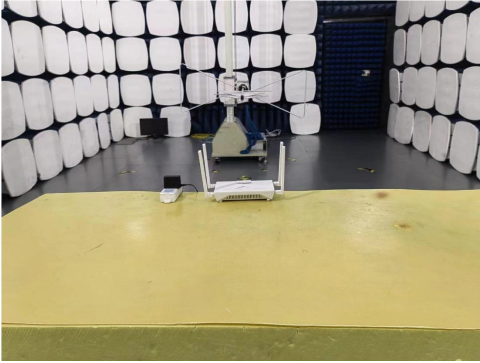
Radiated emission Test Setup (Below 1GHz) Adapter1
