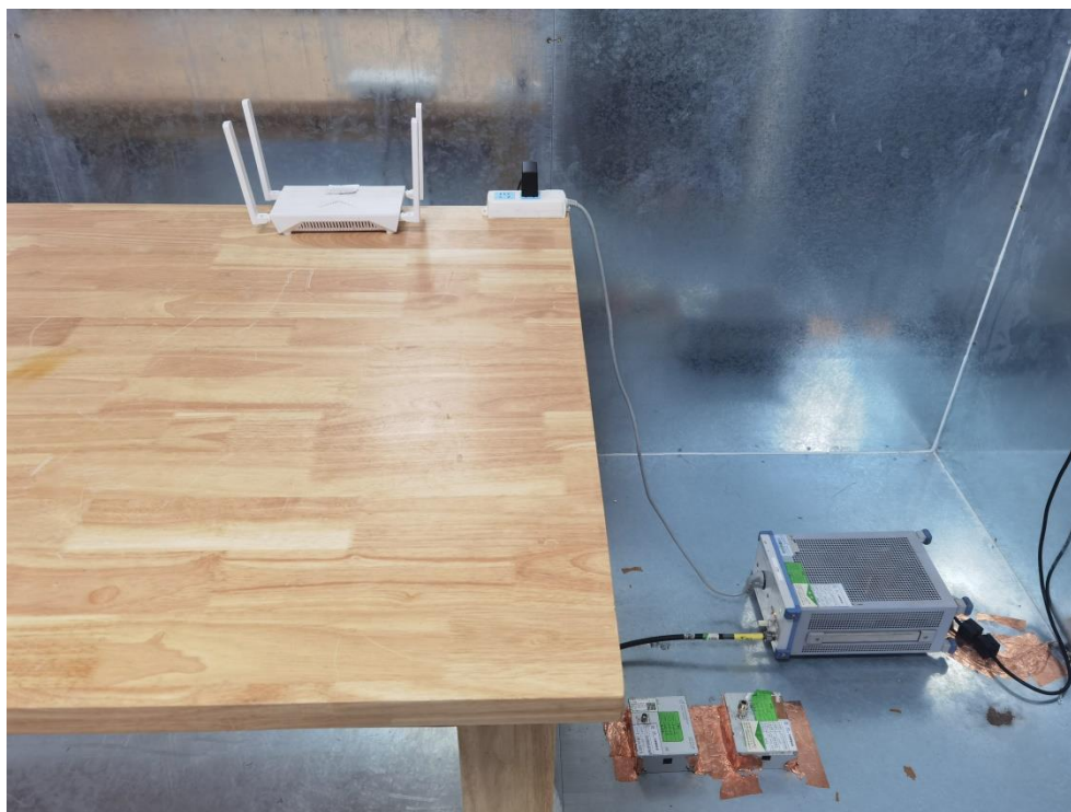
Conducted Emission Test Setup Adapter1
