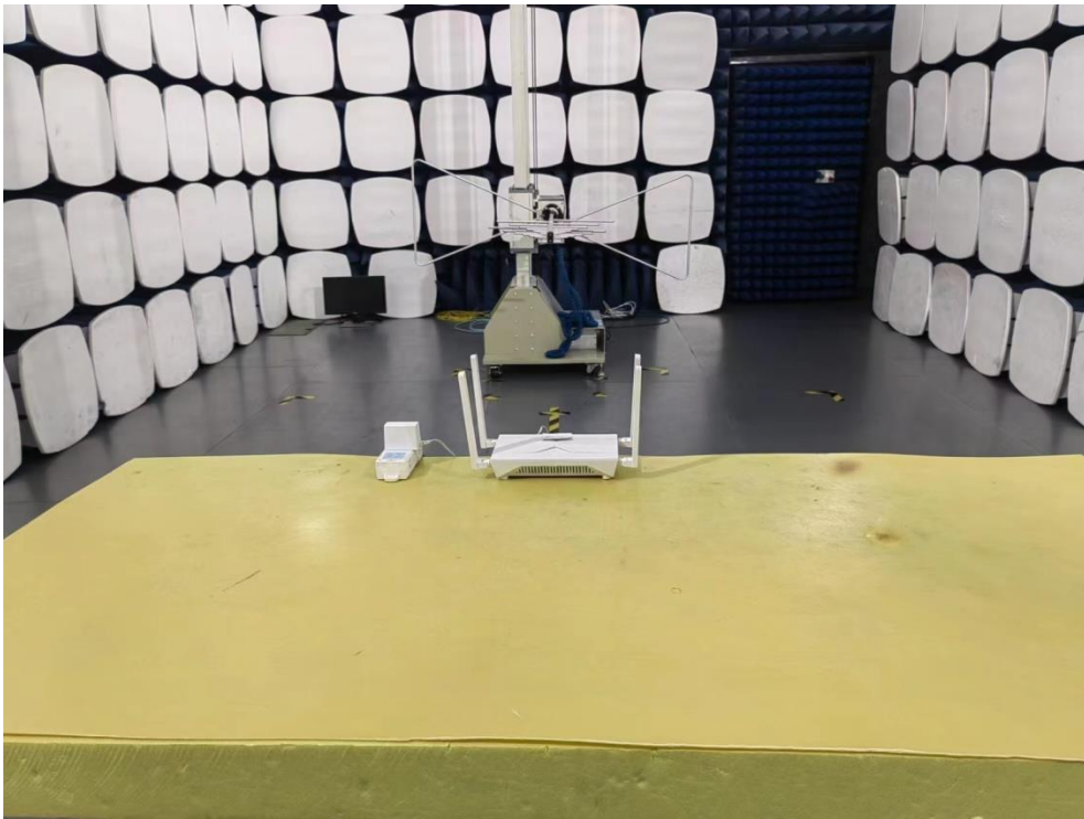
Radiated emission Test Setup (Below 1GHz) Adapter2
