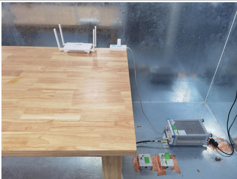
Conducted Emission Test Setup Adapter2
