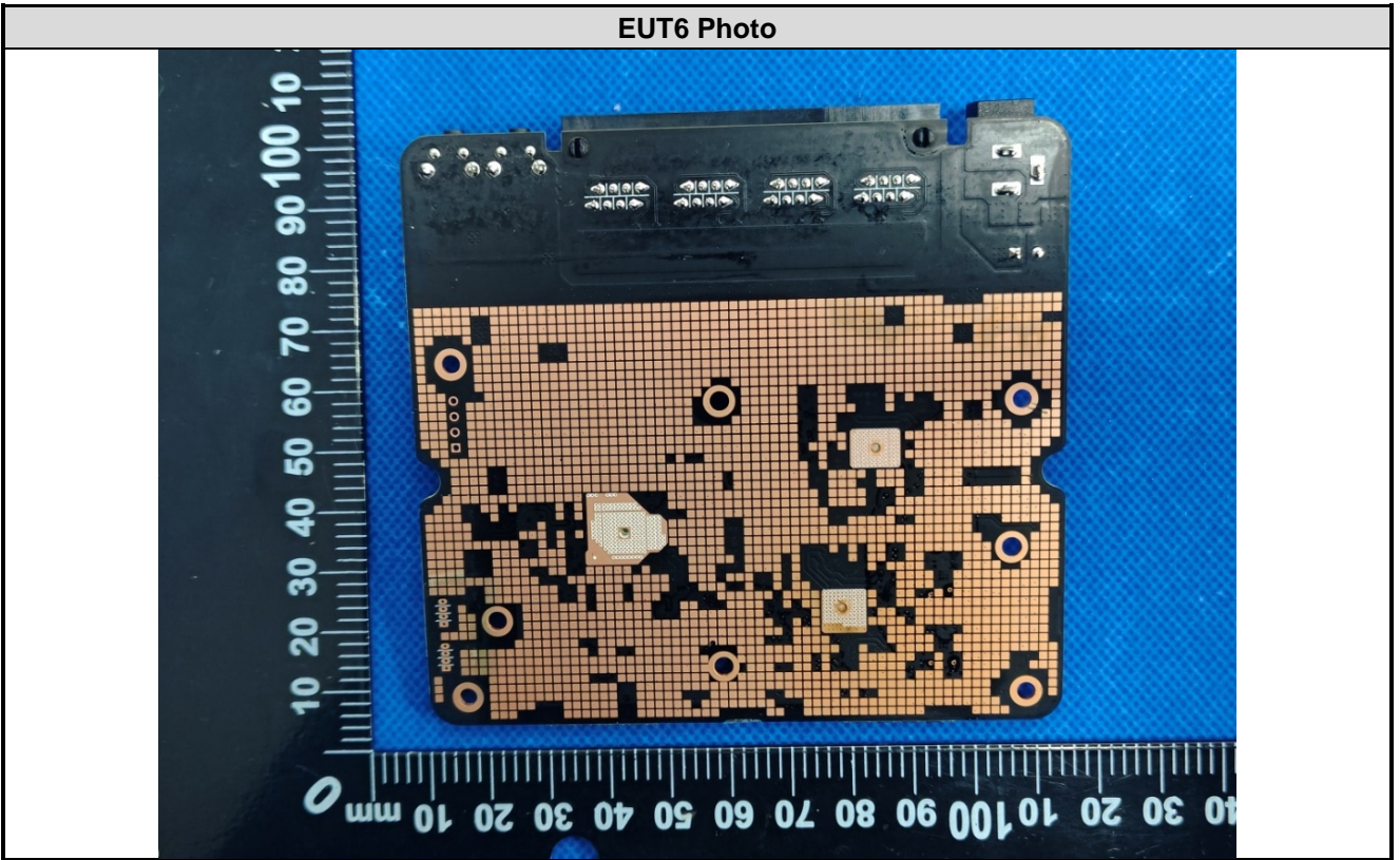
EUT6 Photo
