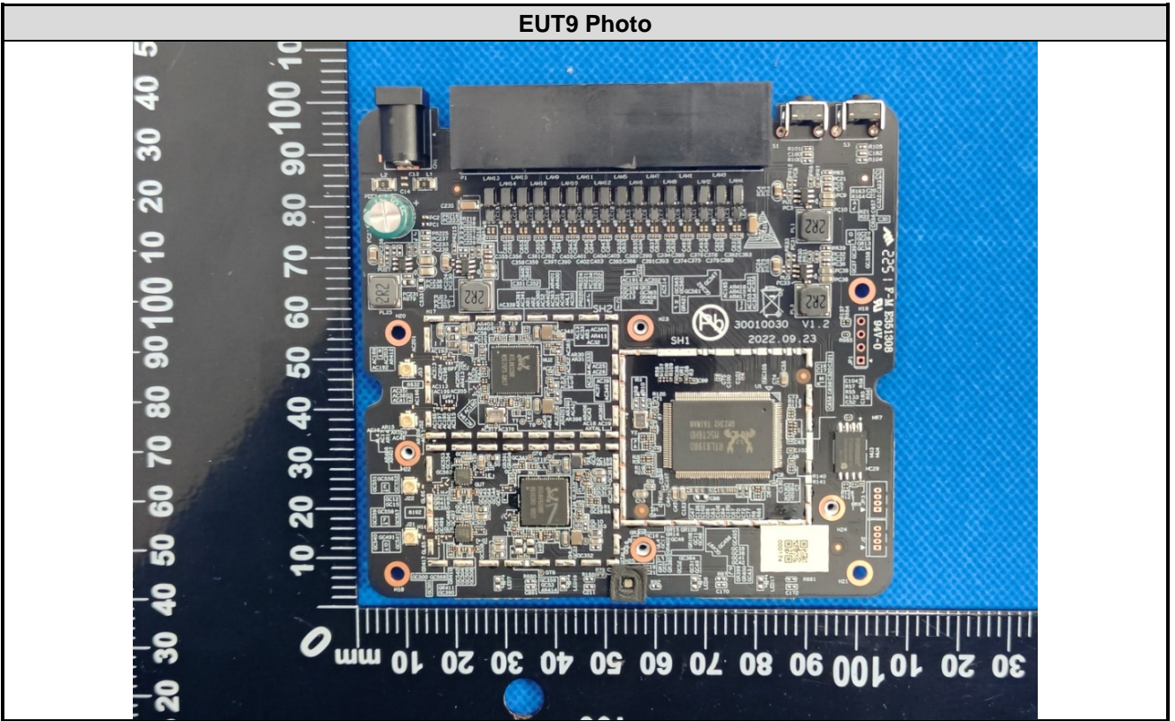
EUT9 Photo
