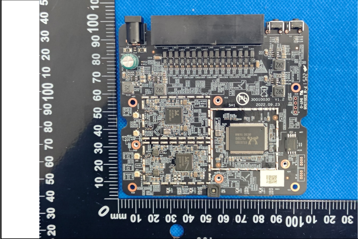
EUT1 Photo
