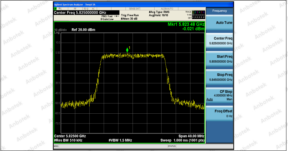
11AC20SISO_Ant2_5825
