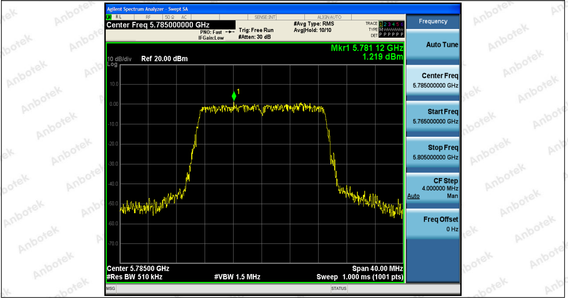
11N20SISO_Ant1_5785
