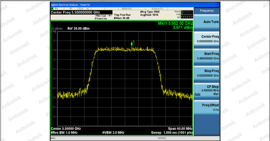
11AC20SISO_Ant2_5500
