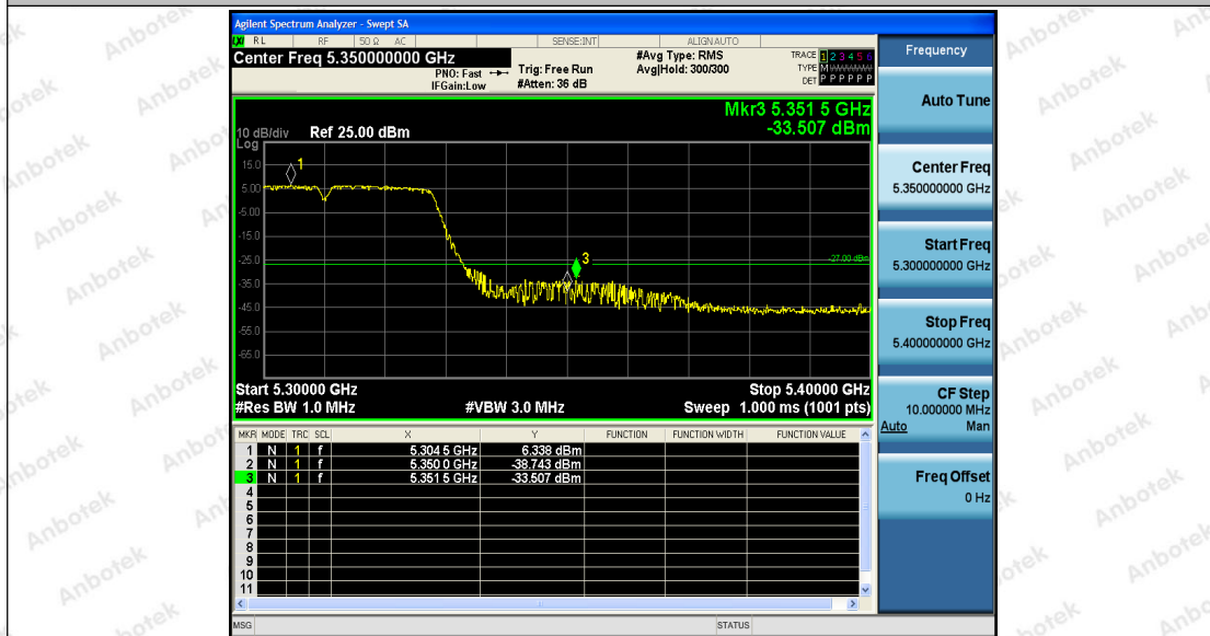
11AC40SISO_Ant1_High_5310
