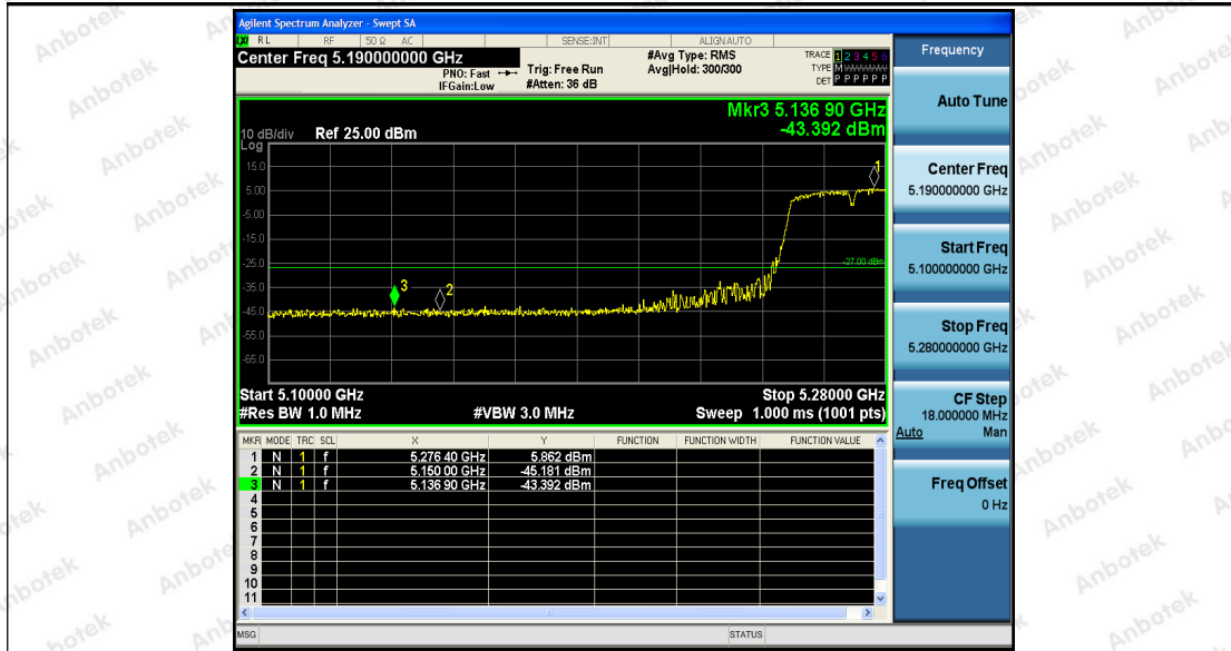
11AC40SISO_Ant2_Low_5270
