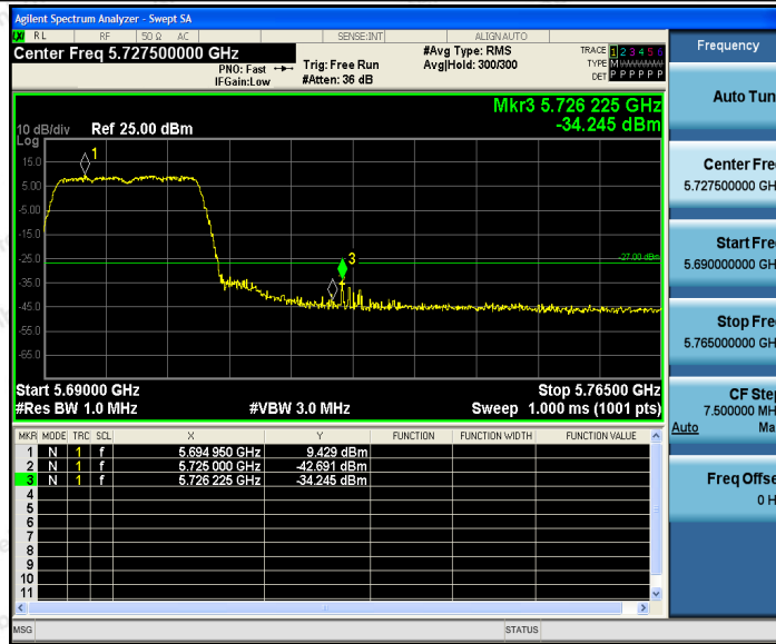
11N20SISO_Ant2_High_5700
