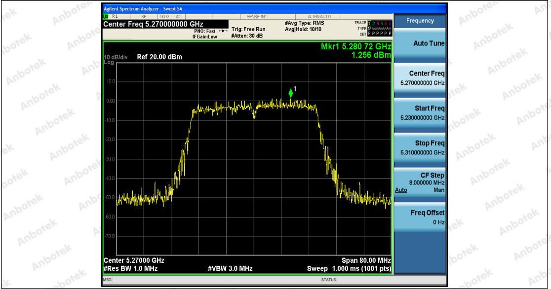
11AC40SISO_Ant1_5270
