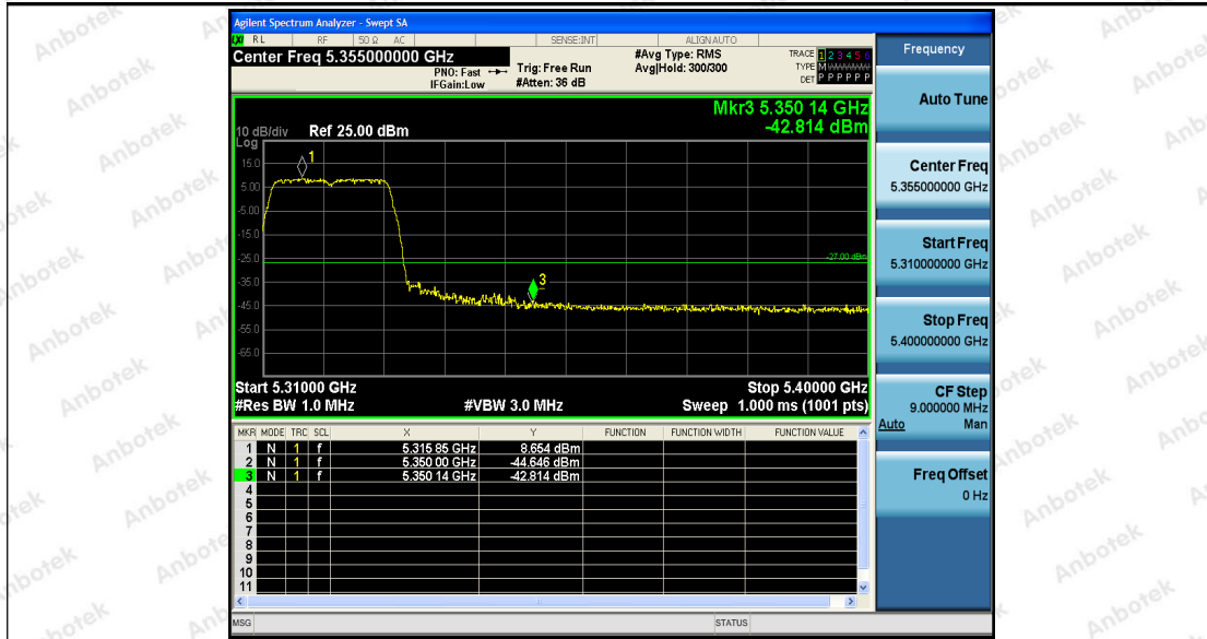
11AC20SISO_Ant2_High_5320
