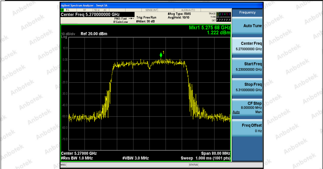
11N40SISO_Ant2_5270
