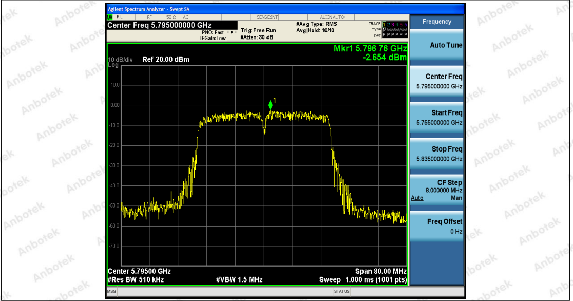
11N40SISO_Ant1_5795
