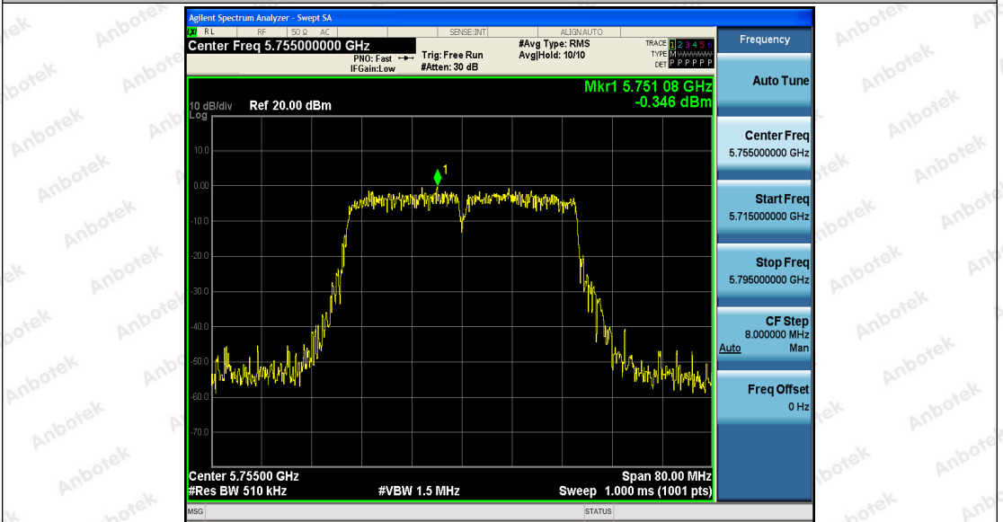
11AC40SISO_Ant1_5755
