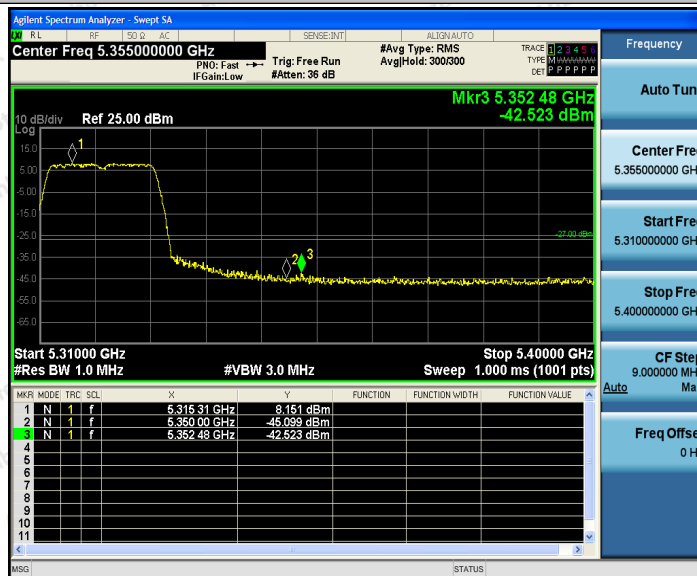
11N20SISO_Ant2_High_5320
