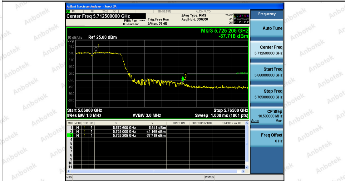
11AC40SISO_Ant2_High_5670
