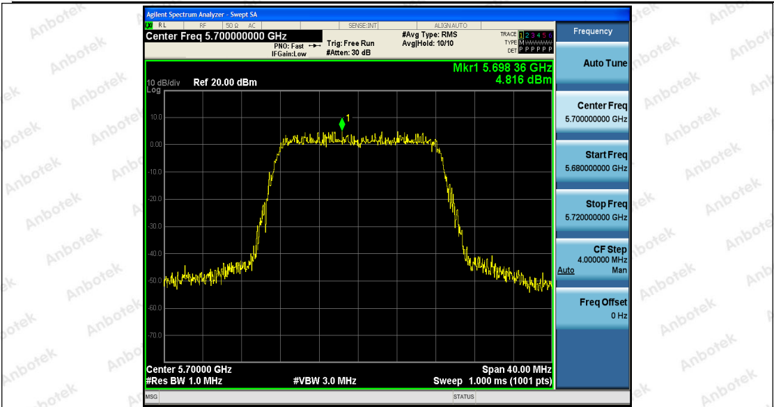
11AC20SISO_Ant2_5700
