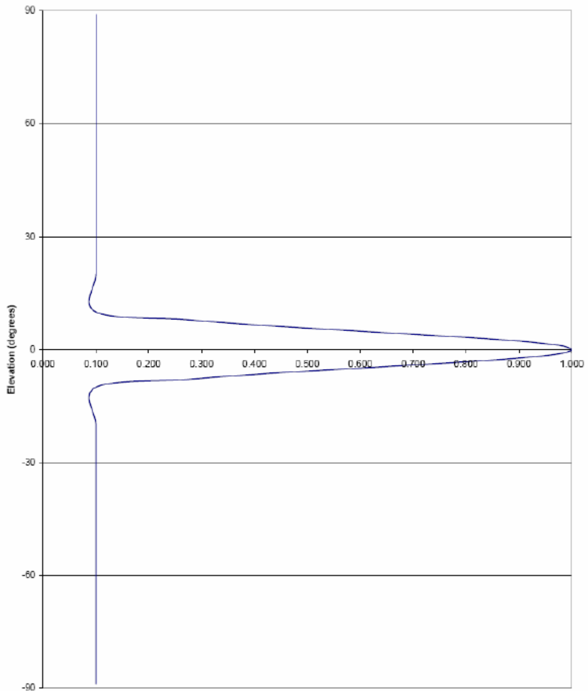
Hub Antenna Elevation Plot Relative Field
