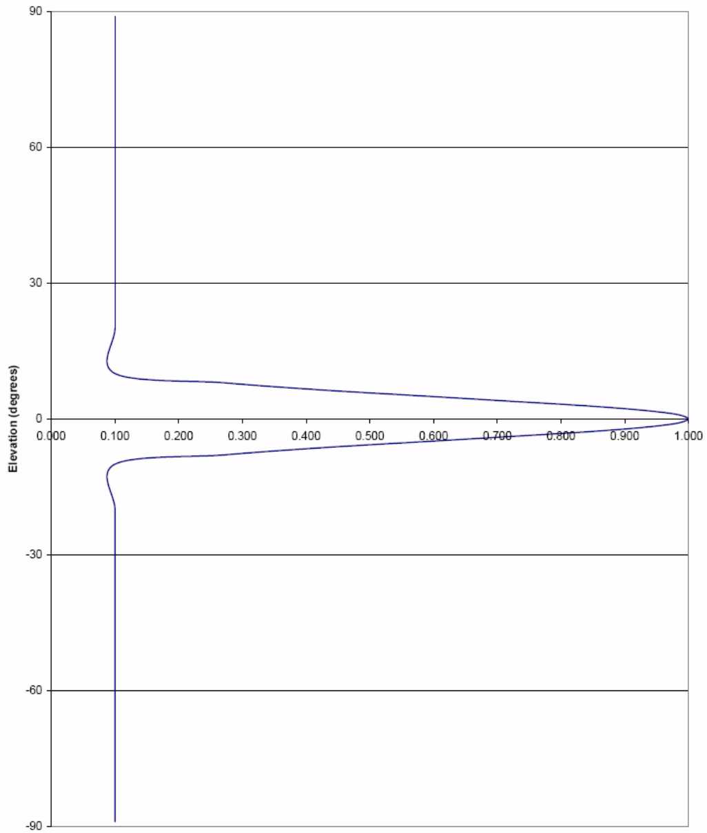
Hub Antenna Elevation Plot Relative Field
