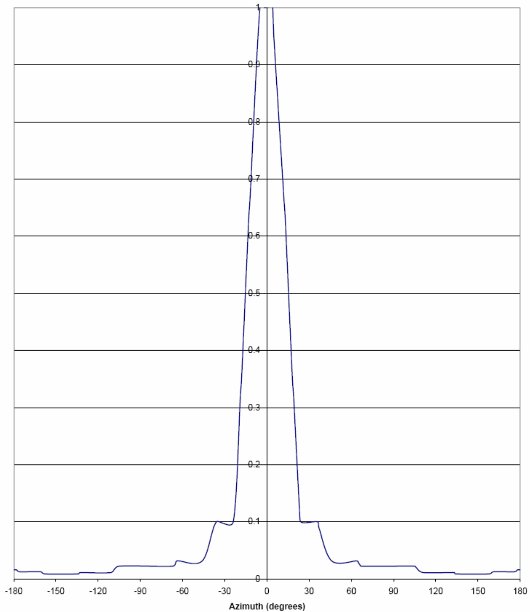
Aperto Customer Terminal Antenna Relative Field Plot Horizontal Plane
