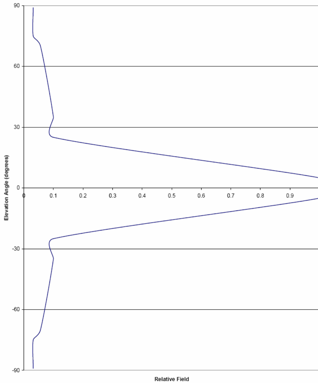
Aperto Customer Terminal Antenna Elevation Pattern
