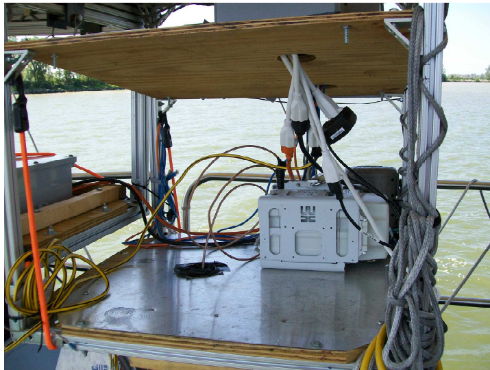
A similar payload bay constructed of 80/20 frame
