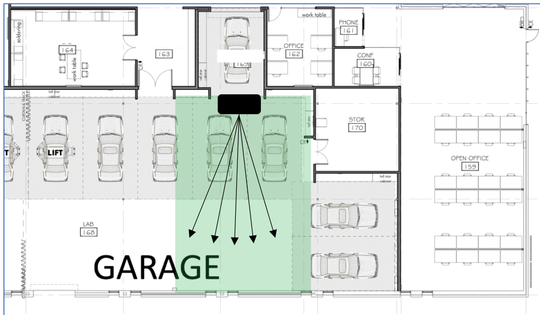
Figure 1. Illustration of planned GPS Repeater orientation at 380 N Pastoria Ave, Sunnyvale CA.
