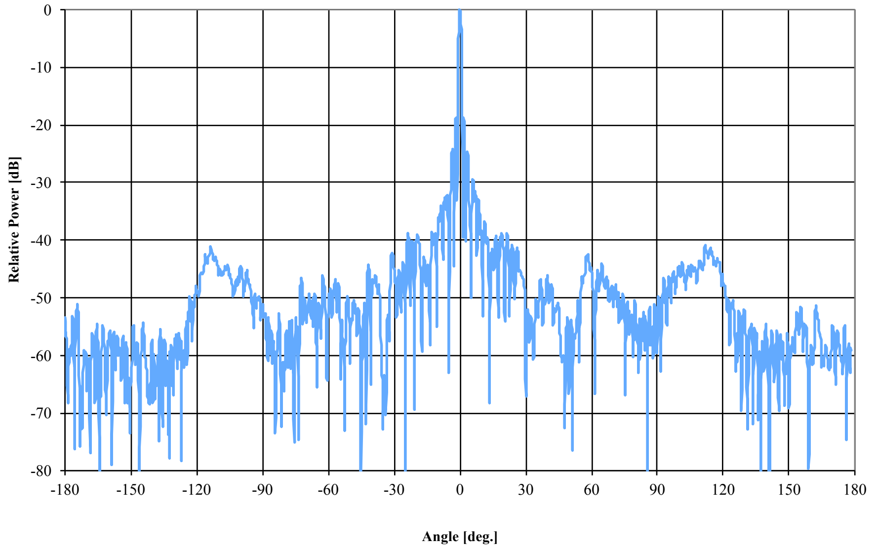
SII 9.1 M P/N 721676-001 Elevation Plane @2.052 GHz Rev: RHC Only Xmit: RHC Grn.Refl.Range Pattern #125254
