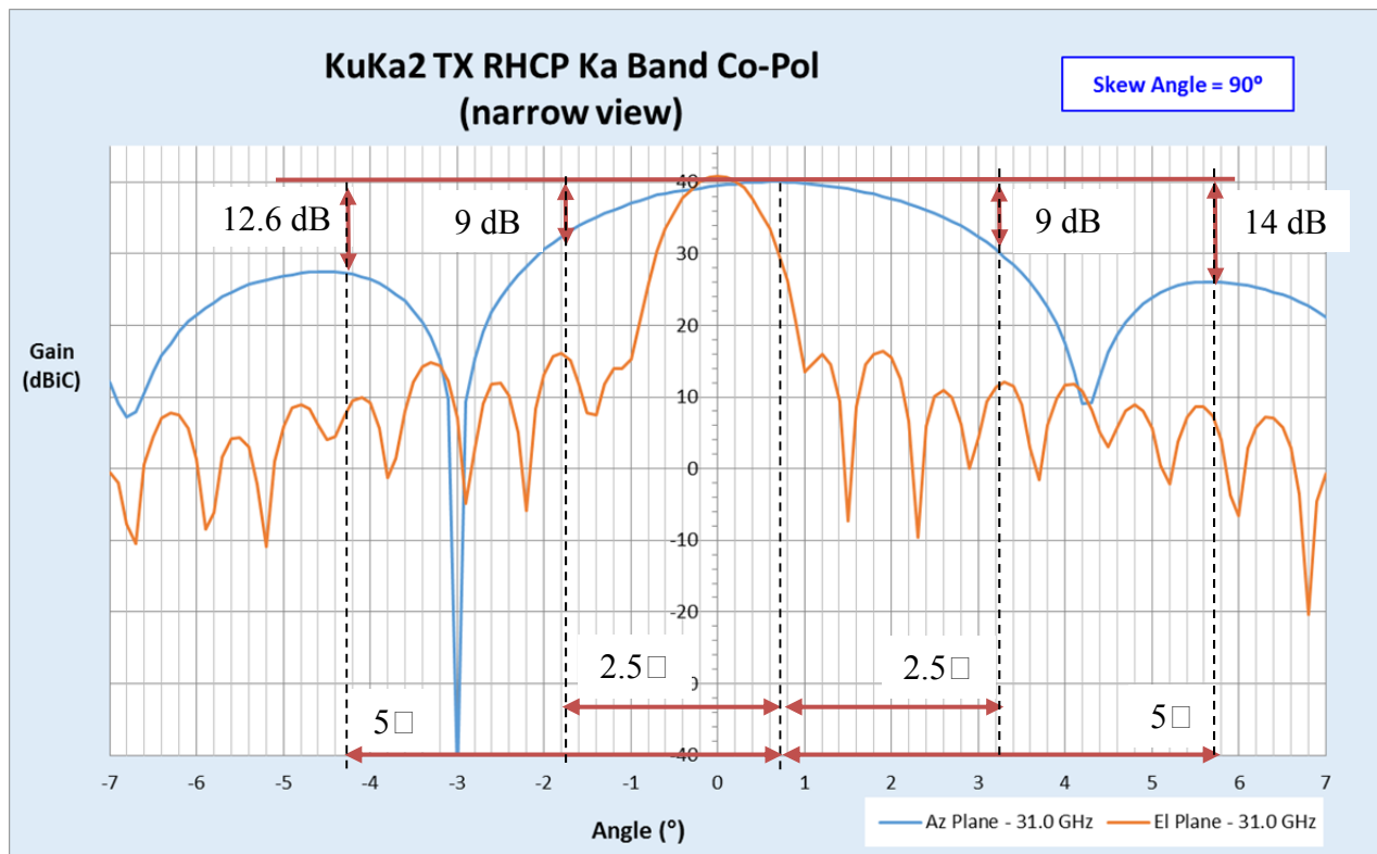
Figure 2: Measured RHCP Transmit Terminal Antenna narrow pattern cuts (+/- 7.0°) for worst case Skew angle 90°. These patterns are measured with radome.
