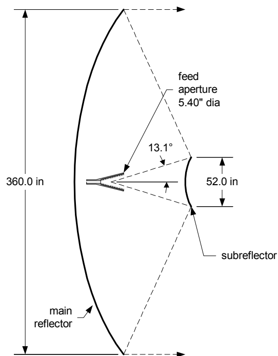
FIGURE 1 - ANTENNA GEOMETRY
