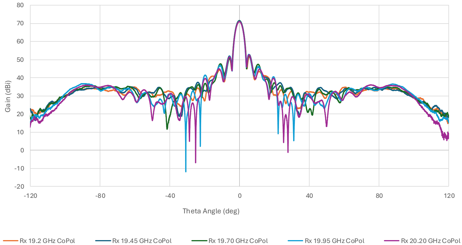
Antenna Receive Gain CoPol 19.2-20.2 GHz
