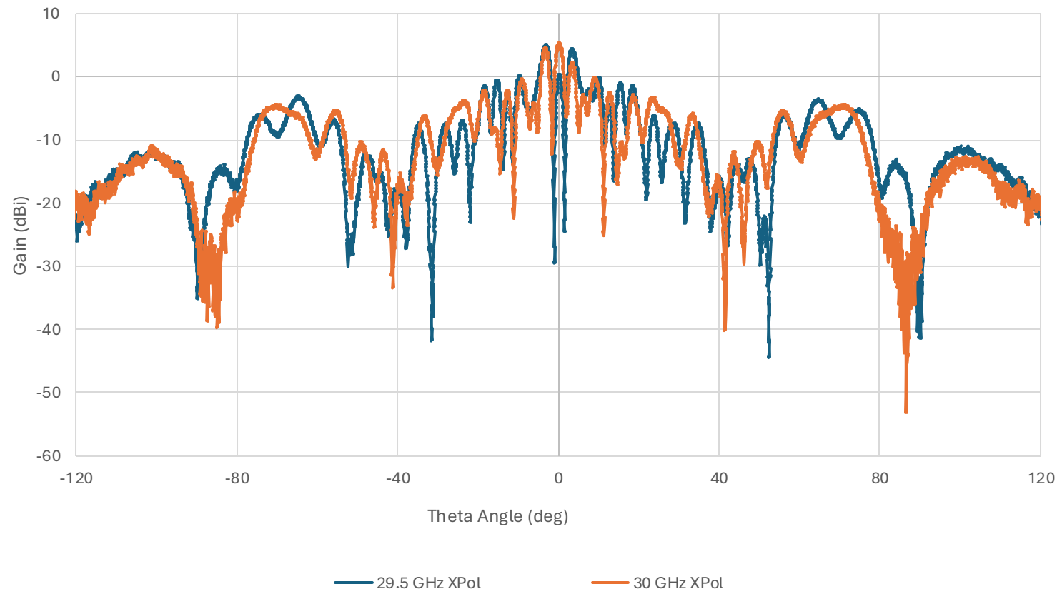
Antenna Transmit Gain CrossPol 29.5-30 GHz
