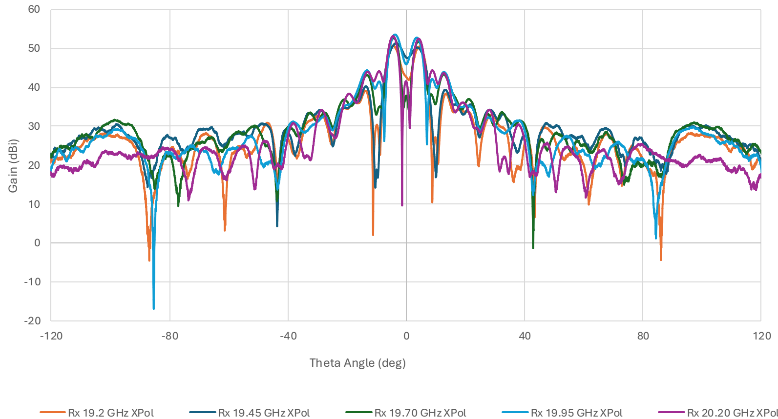
Antenna Receive Gain CrossPol 19.2-20.2 GHz
