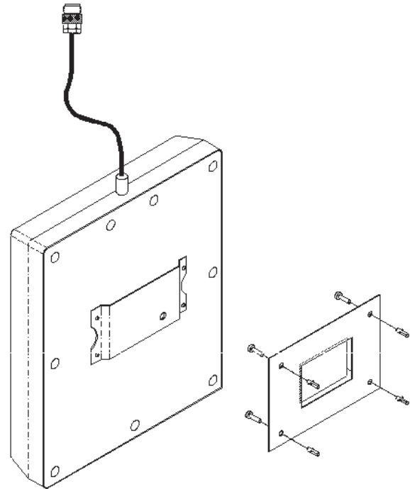
Wall Mounting Configuration
