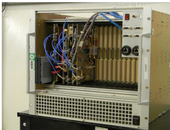
Figure 1. The FlexSAR-X VME chassis.
