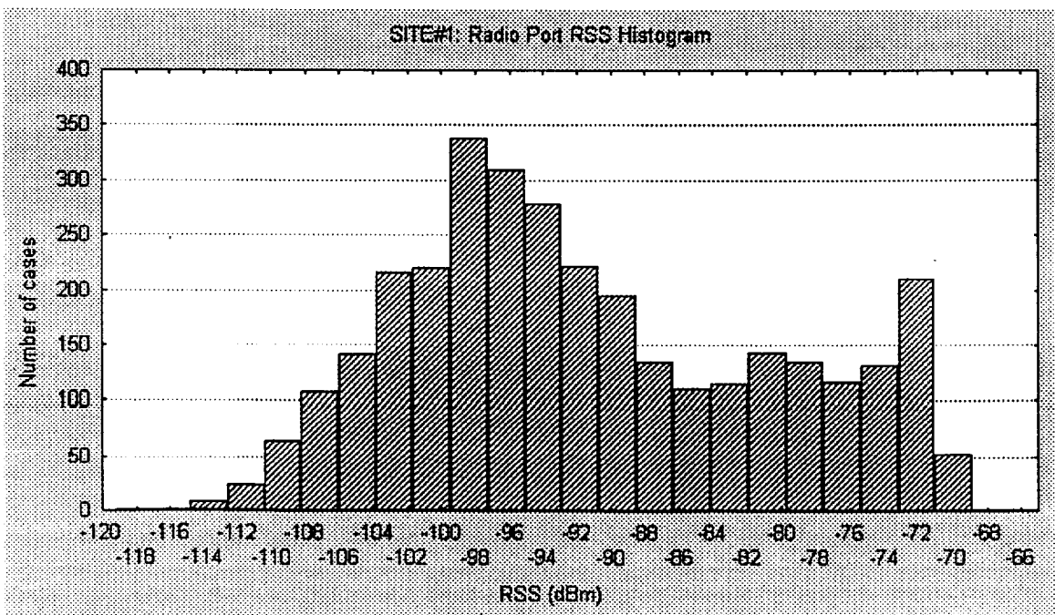
Figure 4.2.1.4. Base Station 1 received signal histogram
