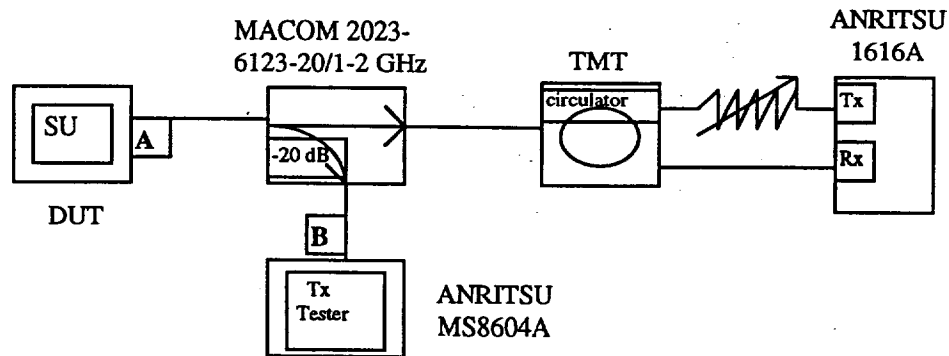
Figure 3.1 Calibration test configuration
