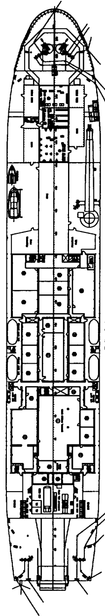
Bulwark Deck
