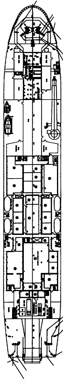
Main Deck
