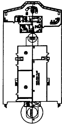
4th Bridge Deck
