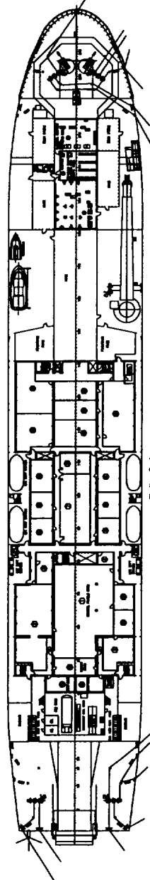
2nd. Bridge Deck
