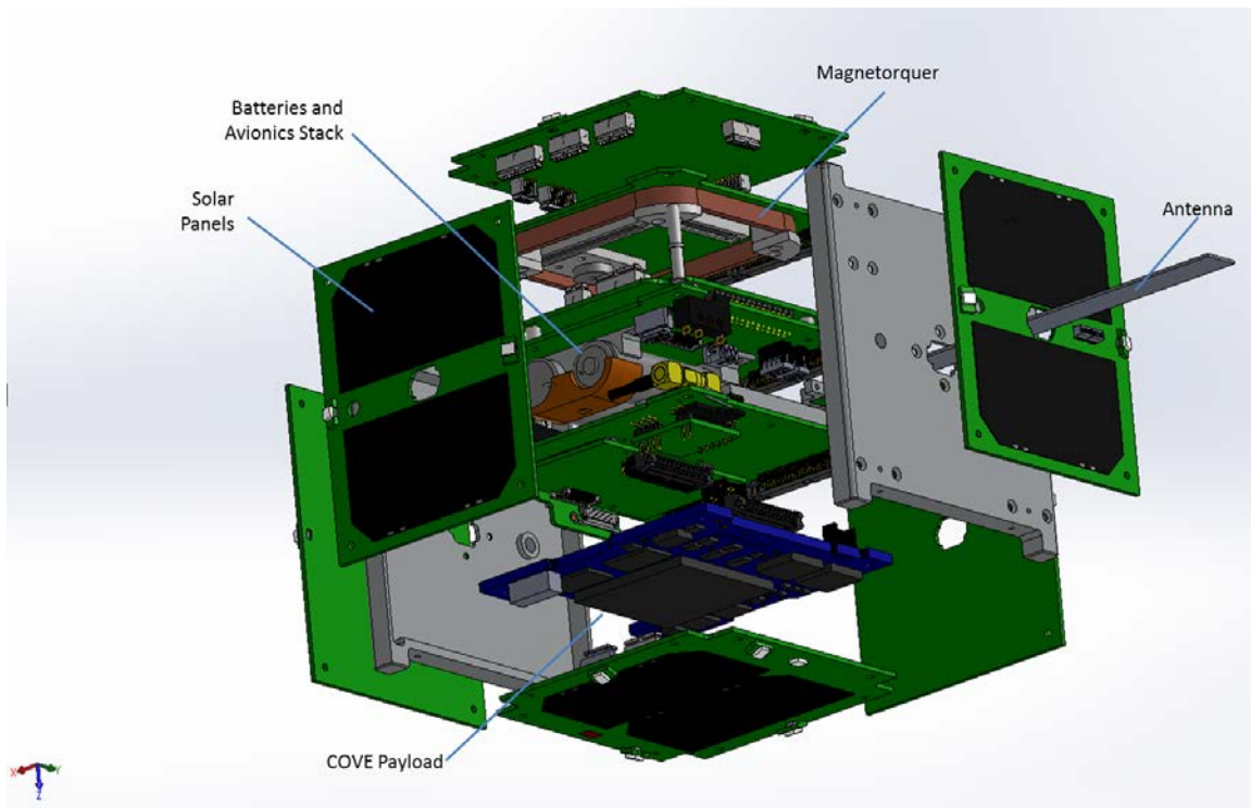
Figure 2: MCubed-II Expanded View
