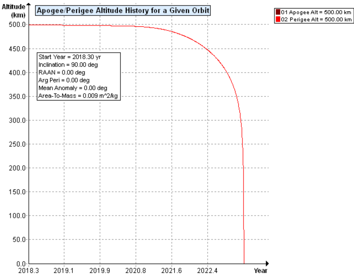
Figure 3: TechEdSat-7 Orbit History for Case 2: Failed Deployment
